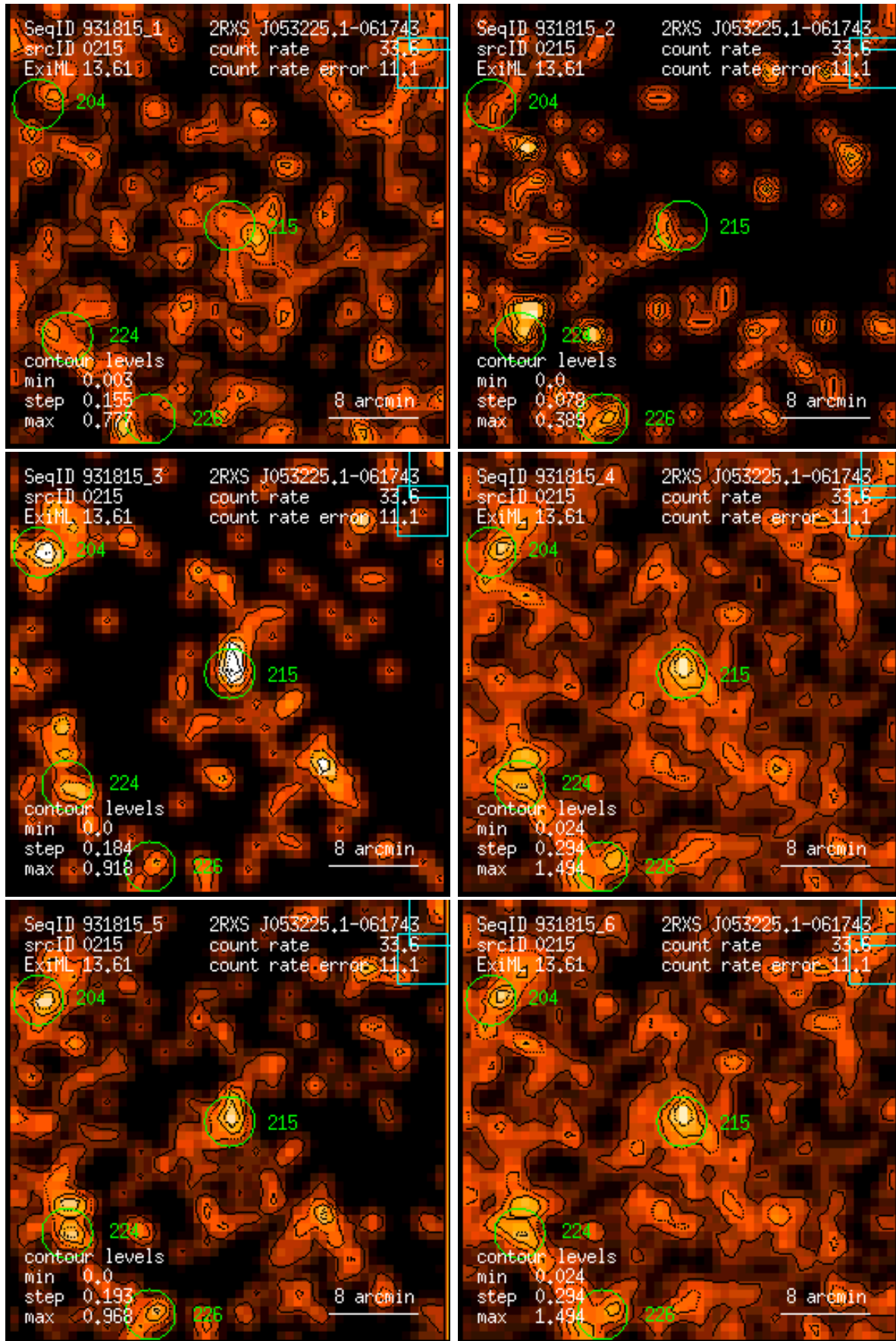
Figure 215: RASS 931815: detection 0215: band rate images, Gaussian filter: (1) PSPC channels 11 – 41, (2) 52 – 90, (3) 91 – 201, (4) 11 – 235, (5) 52 – 201, (6) 11 – 201. Broad band rates in counts/ks. Band rate contour levels in counts/ks/arcmin 2 .
