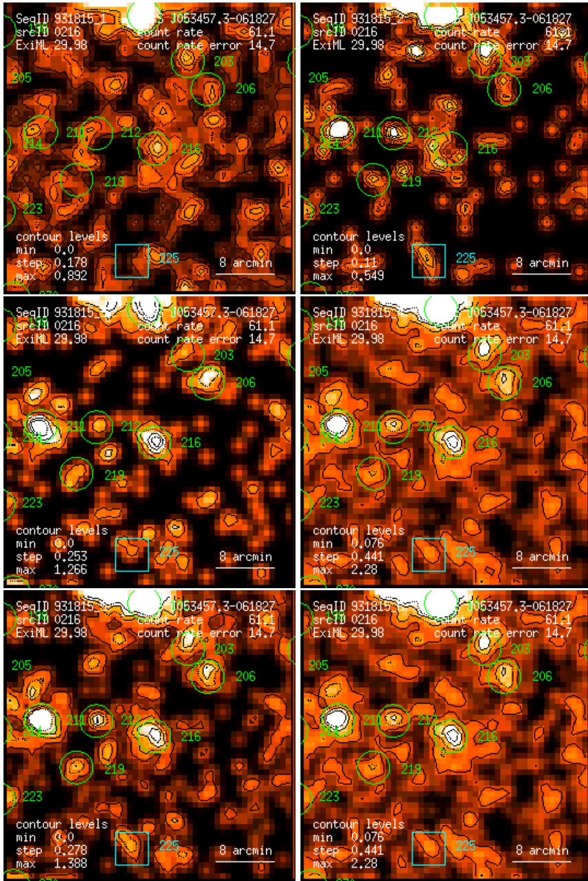
Figure 216: RASS 931815: detection 0216: band rate images, Gaussian filter: (1) PSPC channels 11 – 41, (2) 52 – 90, (3) 91 – 201, (4) 11 – 235, (5) 52 – 201, (6) 11 – 201. Broad band rates in counts/ks. Band rate contour levels in counts/ks/arcmin 2 .
