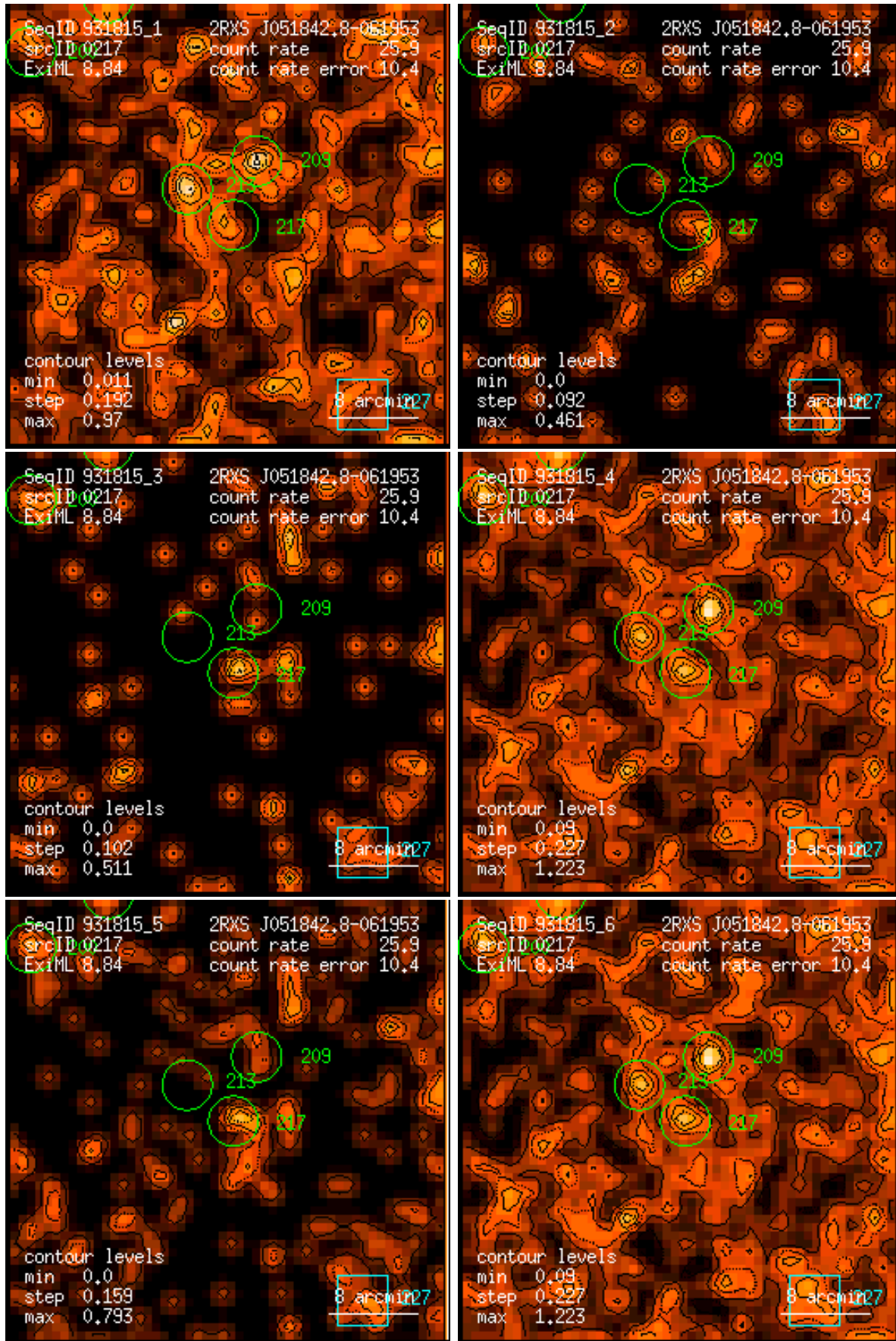
Figure 217: RASS 931815: detection 0217: band rate images, Gaussian filter: (1) PSPC channels 11 – 41, (2) 52 – 90, (3) 91 – 201, (4) 11 – 235, (5) 52 – 201, (6) 11 – 201. Broad band rates in counts/ks. Band rate contour levels in counts/ks/arcmin 2 .
