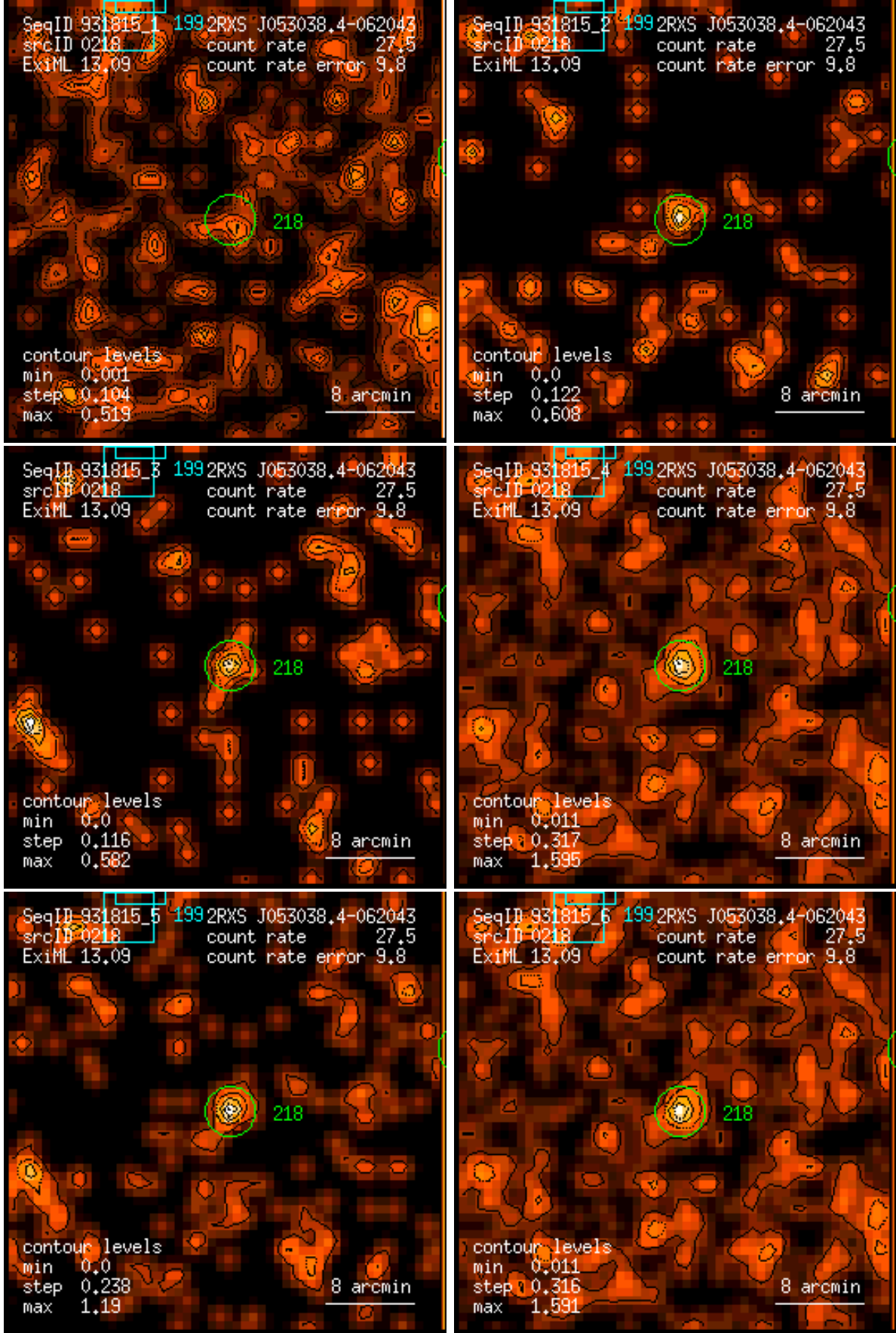
Figure 218: RASS 931815: detection 0218: band rate images, Gaussian filter: (1) PSPC channels 11 – 41, (2) 52 – 90, (3) 91 – 201, (4) 11 – 235, (5) 52 – 201, (6) 11 – 201. Broad band rates in counts/ks. Band rate contour levels in counts/ks/arcmin 2 .
