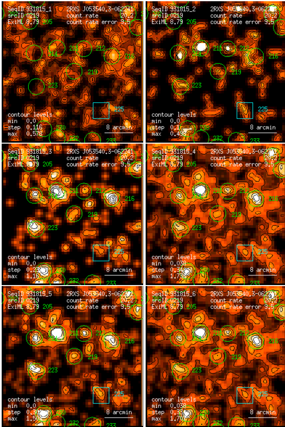
Figure 219: RASS 931815: detection 0219: band rate images, Gaussian filter: (1) PSPC channels 11 – 41, (2) 52 – 90, (3) 91 – 201, (4) 11 – 235, (5) 52 – 201, (6) 11 – 201. Broad band rates in counts/ks. Band rate contour levels in counts/ks/arcmin 2 .
