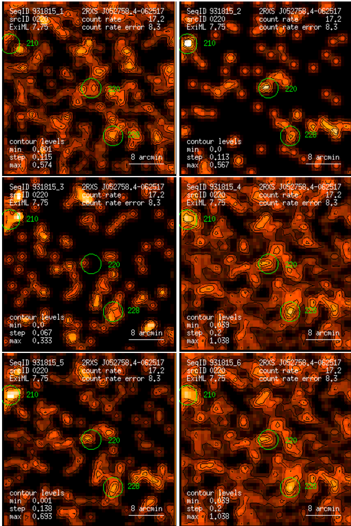
Figure 220: RASS 931815: detection 0220: band rate images, Gaussian filter: (1) PSPC channels 11 – 41, (2) 52 – 90, (3) 91 – 201, (4) 11 – 235, (5) 52 – 201, (6) 11 – 201. Broad band rates in counts/ks. Band rate contour levels in counts/ks/arcmin 2 .
