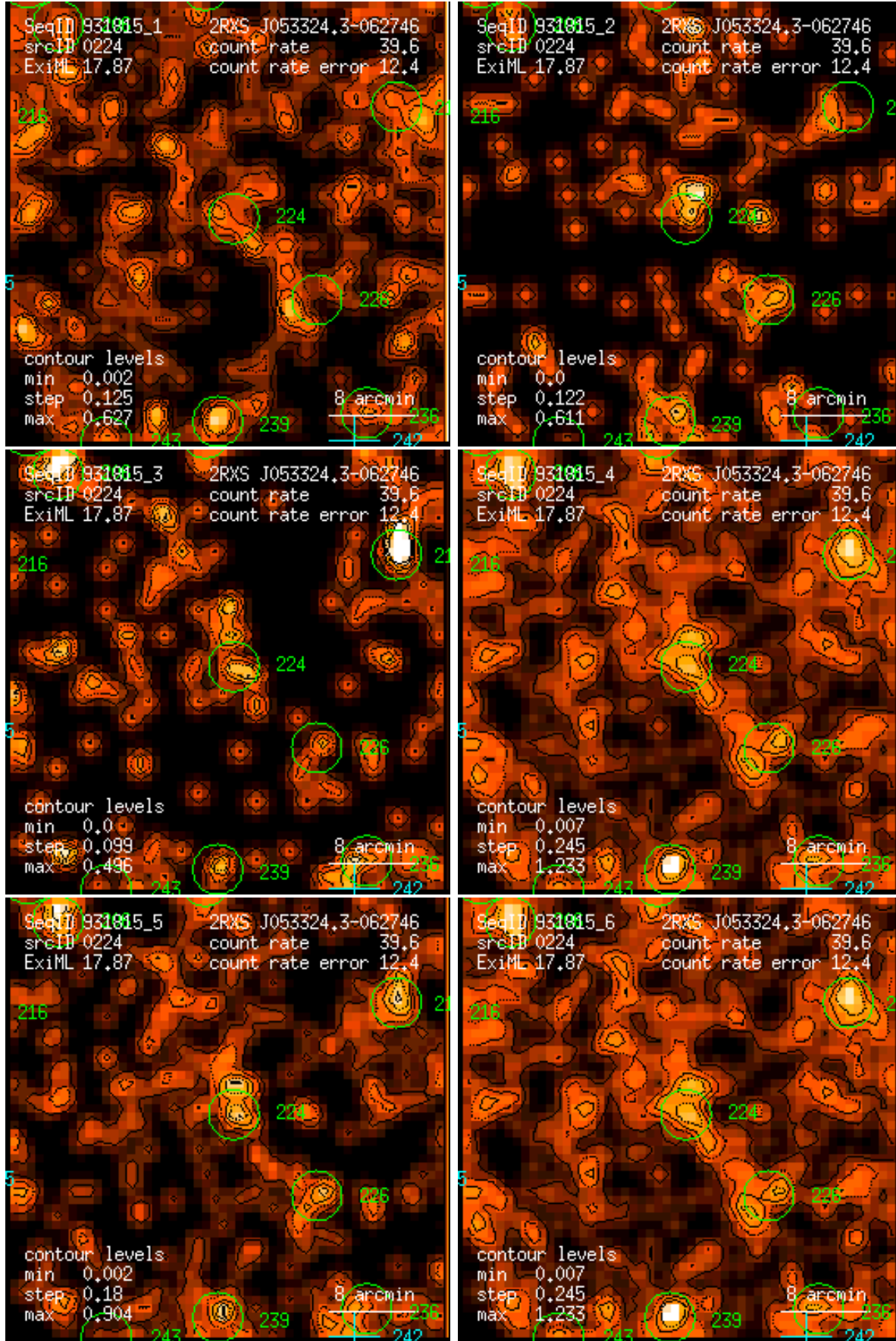
Figure 224: RASS 931815: detection 0224: band rate images, Gaussian filter: (1) PSPC channels 11 – 41, (2) 52 – 90, (3) 91 – 201, (4) 11 – 235, (5) 52 – 201, (6) 11 – 201. Broad band rates in counts/ks. Band rate contour levels in counts/ks/arcmin 2 .
