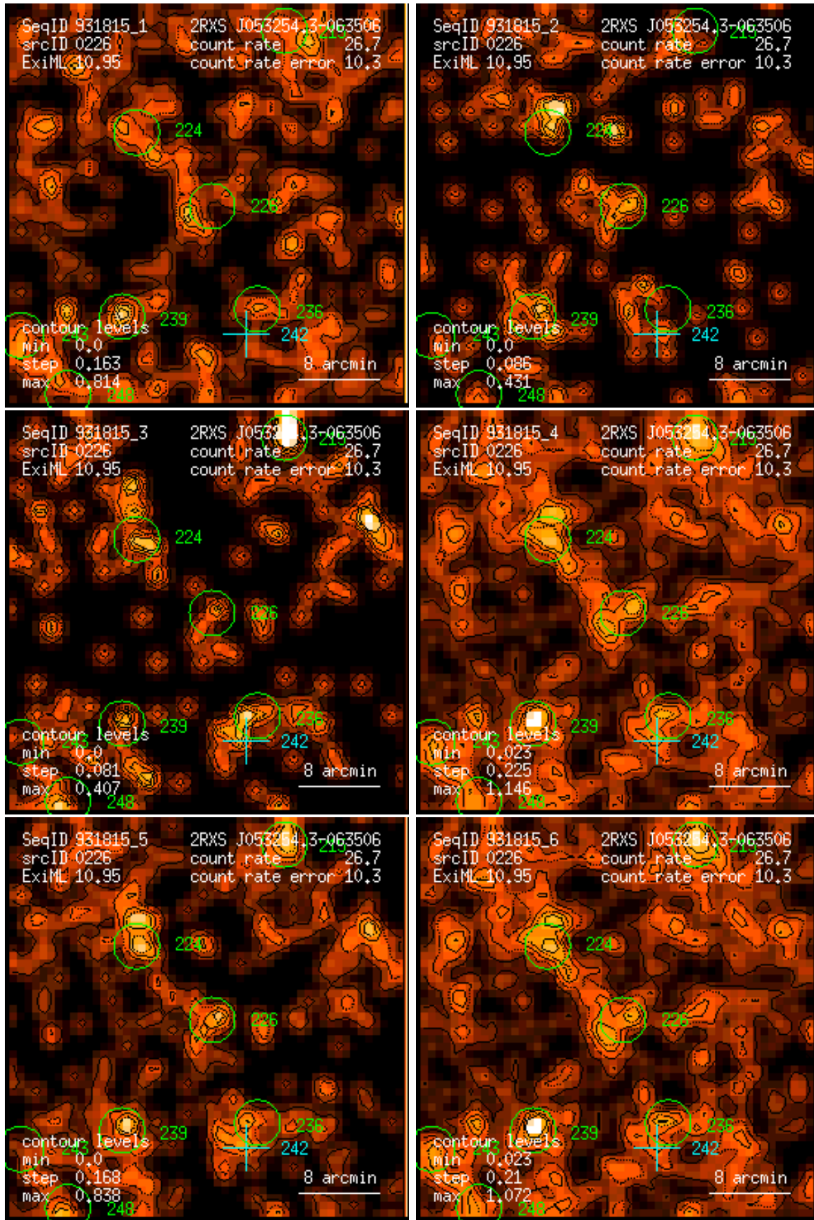
Figure 226: RASS 931815: detection 0226: band rate images, Gaussian filter: (1) PSPC channels 11 – 41, (2) 52 – 90, (3) 91 – 201, (4) 11 – 235, (5) 52 – 201, (6) 11 – 201. Broad band rates in counts/ks. Band rate contour levels in counts/ks/arcmin 2 .
