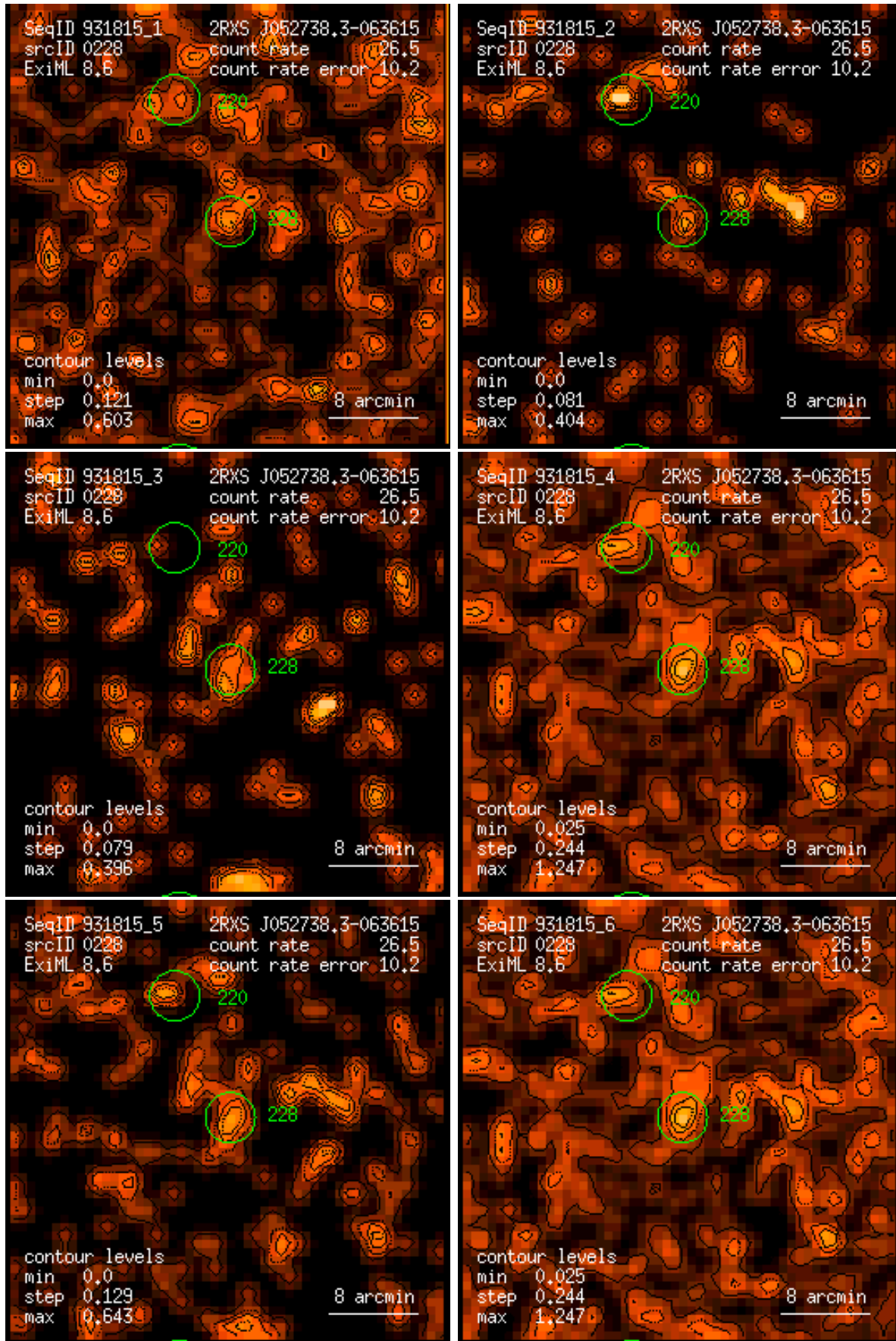
Figure 228: RASS 931815: detection 0228: band rate images, Gaussian filter: (1) PSPC channels 11 – 41, (2) 52 – 90, (3) 91 – 201, (4) 11 – 235, (5) 52 – 201, (6) 11 – 201. Broad band rates in counts/ks. Band rate contour levels in counts/ks/arcmin 2 .
