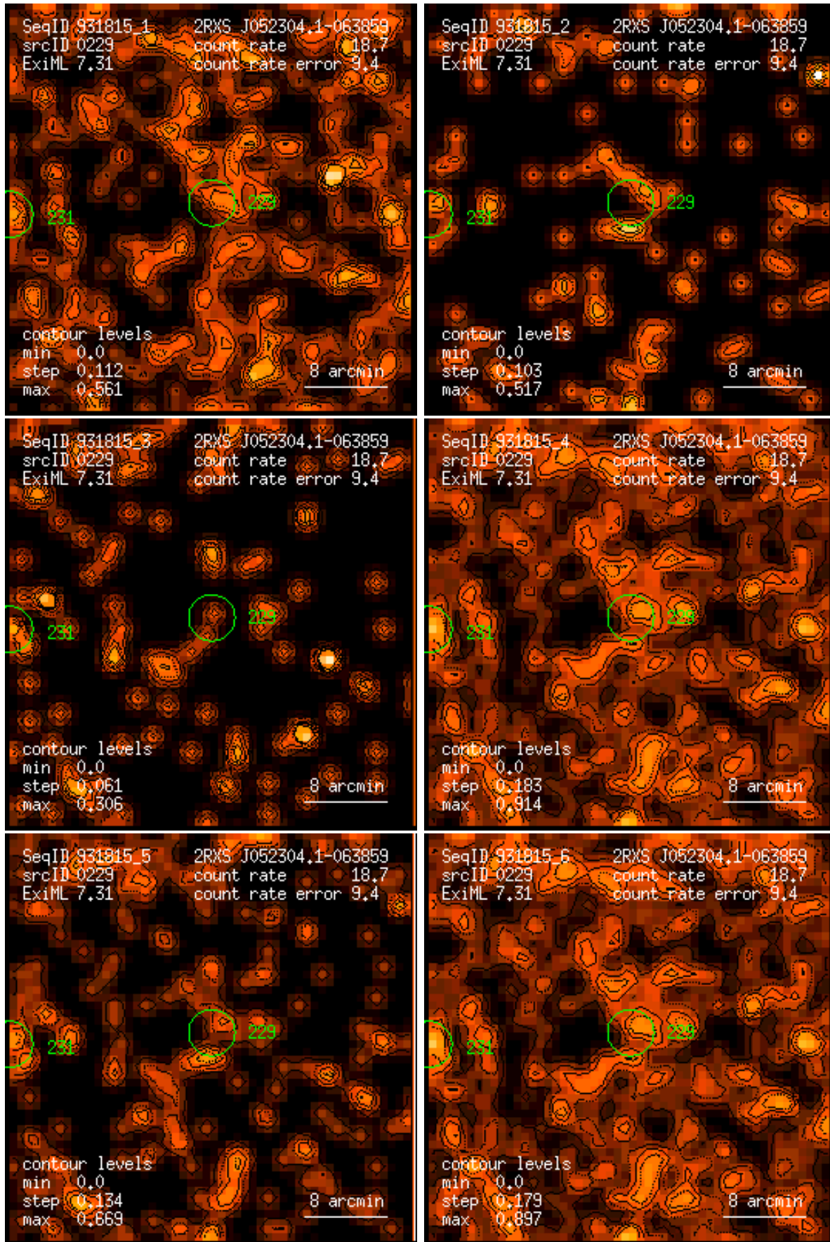
Figure 229: RASS 931815: detection 0229: band rate images, Gaussian filter: (1) PSPC channels 11 – 41, (2) 52 – 90, (3) 91 – 201, (4) 11 – 235, (5) 52 – 201, (6) 11 – 201. Broad band rates in counts/ks. Band rate contour levels in counts/ks/arcmin 2 .
