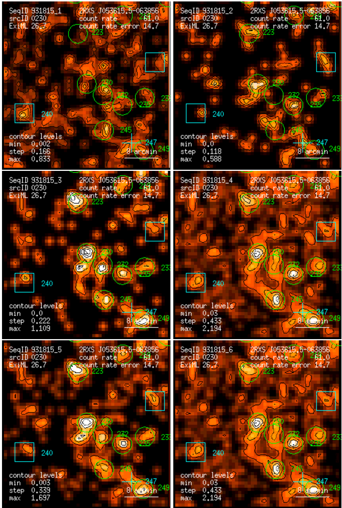
Figure 230: RASS 931815: detection 0230: band rate images, Gaussian filter: (1) PSPC channels 11 – 41, (2) 52 – 90, (3) 91 – 201, (4) 11 – 235, (5) 52 – 201, (6) 11 – 201. Broad band rates in counts/ks. Band rate contour levels in counts/ks/arcmin 2 .
