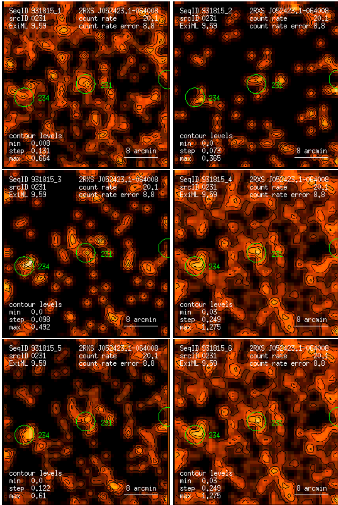
Figure 231: RASS 931815: detection 0231: band rate images, Gaussian filter: (1) PSPC channels 11 – 41, (2) 52 – 90, (3) 91 – 201, (4) 11 – 235, (5) 52 – 201, (6) 11 – 201. Broad band rates in counts/ks. Band rate contour levels in counts/ks/arcmin 2 .
