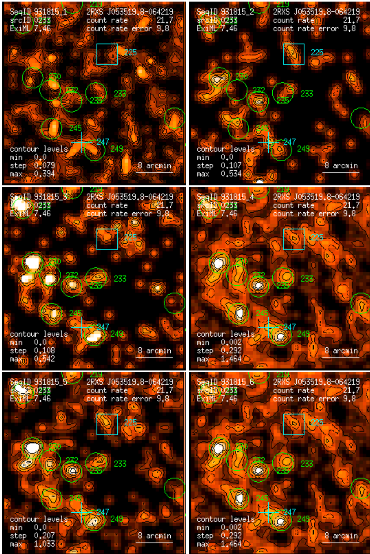
Figure 233: RASS 931815: detection 0233: band rate images, Gaussian filter: (1) PSPC channels 11 – 41, (2) 52 – 90, (3) 91 – 201, (4) 11 – 235, (5) 52 – 201, (6) 11 – 201. Broad band rates in counts/ks. Band rate contour levels in counts/ks/arcmin 2 .
