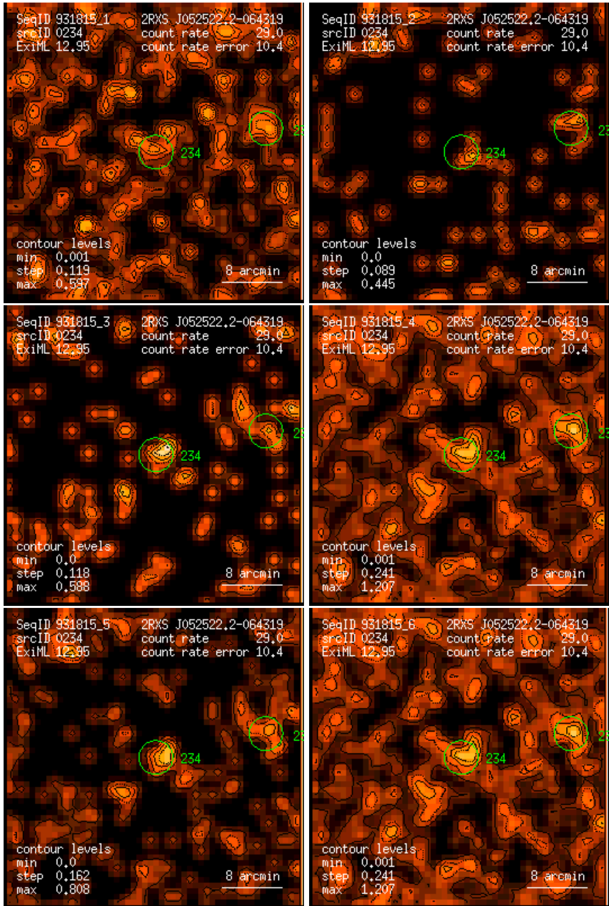
Figure 234: RASS 931815: detection 0234: band rate images, Gaussian filter: (1) PSPC channels 11 – 41, (2) 52 – 90, (3) 91 – 201, (4) 11 – 235, (5) 52 – 201, (6) 11 – 201. Broad band rates in counts/ks. Band rate contour levels in counts/ks/arcmin 2 .
