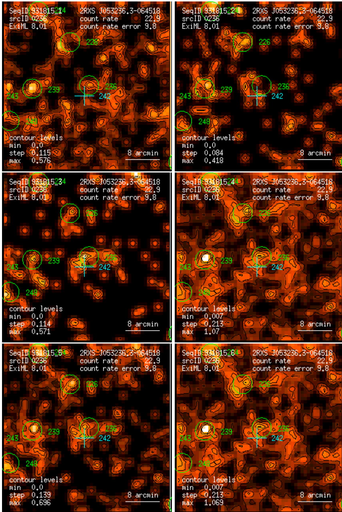
Figure 236: RASS 931815: detection 0236: band rate images, Gaussian filter: (1) PSPC channels 11 – 41, (2) 52 – 90, (3) 91 – 201, (4) 11 – 235, (5) 52 – 201, (6) 11 – 201. Broad band rates in counts/ks. Band rate contour levels in counts/ks/arcmin 2 .
