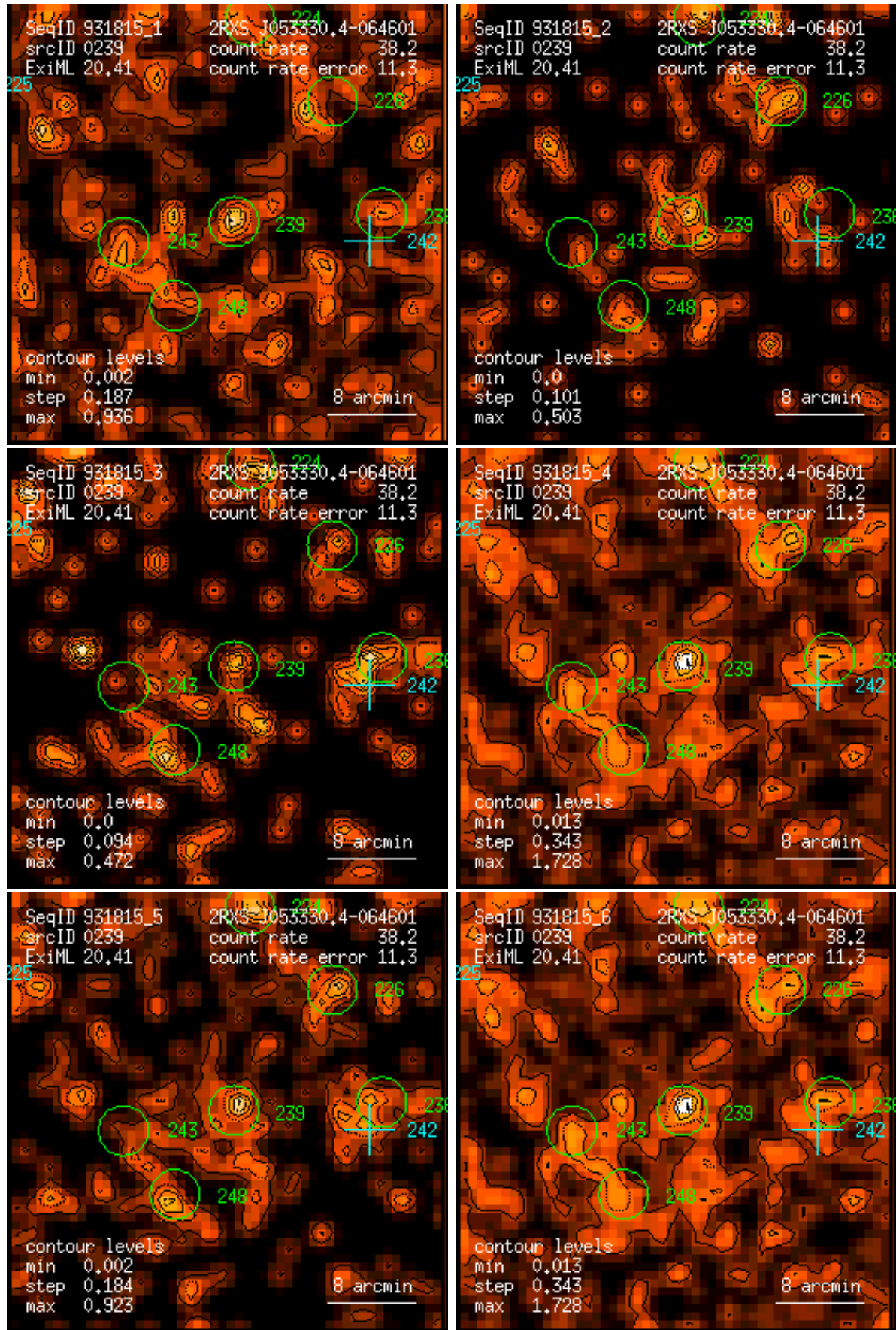
Figure 239: RASS 931815: detection 0239: band rate images, Gaussian filter: (1) PSPC channels 11 – 41, (2) 52 – 90, (3) 91 – 201, (4) 11 – 235, (5) 52 – 201, (6) 11 – 201. Broad band rates in counts/ks. Band rate contour levels in counts/ks/arcmin 2 .
