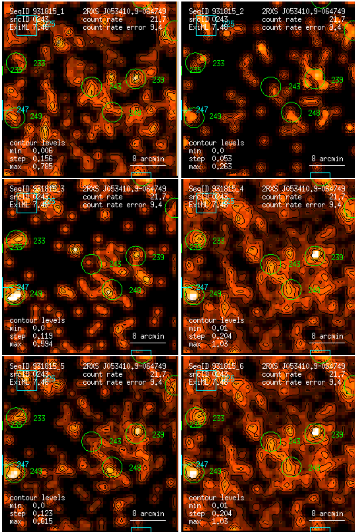
Figure 243: RASS 931815: detection 0243: band rate images, Gaussian filter: (1) PSPC channels 11 – 41, (2) 52 – 90, (3) 91 – 201, (4) 11 – 235, (5) 52 – 201, (6) 11 – 201. Broad band rates in counts/ks. Band rate contour levels in counts/ks/arcmin 2 .
