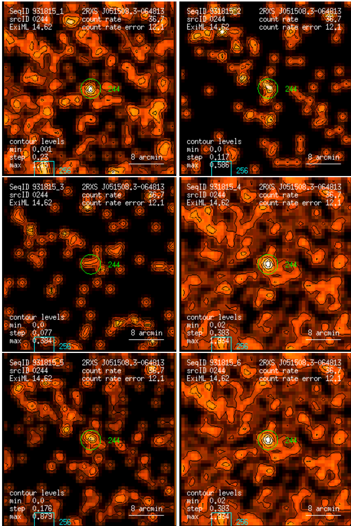
Figure 244: RASS 931815: detection 0244: band rate images, Gaussian filter: (1) PSPC channels 11 – 41, (2) 52 – 90, (3) 91 – 201, (4) 11 – 235, (5) 52 – 201, (6) 11 – 201. Broad band rates in counts/ks. Band rate contour levels in counts/ks/arcmin 2 .
