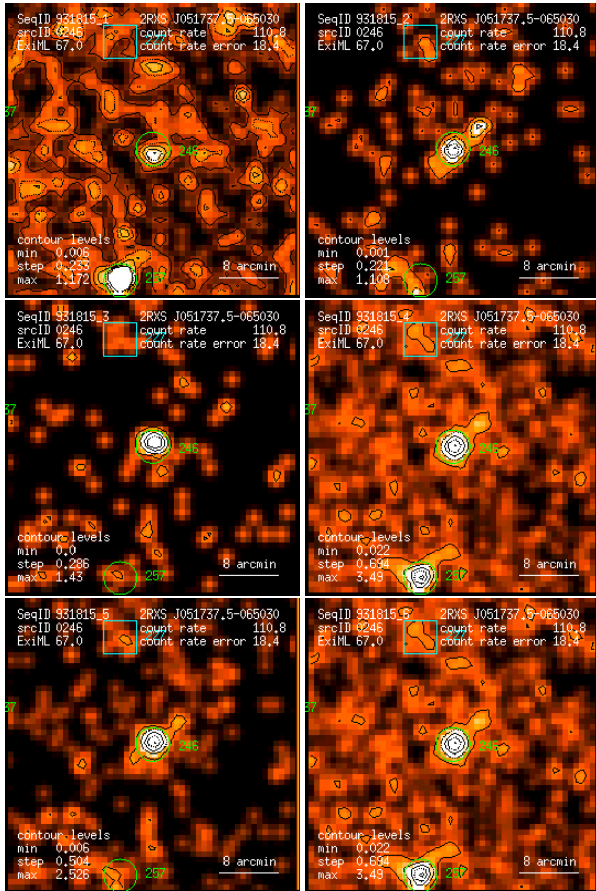
Figure 246: RASS 931815: detection 0246: band rate images, Gaussian filter: (1) PSPC channels 11 – 41, (2) 52 – 90, (3) 91 – 201, (4) 11 – 235, (5) 52 – 201, (6) 11 – 201. Broad band rates in counts/ks. Band rate contour levels in counts/ks/arcmin 2 .
