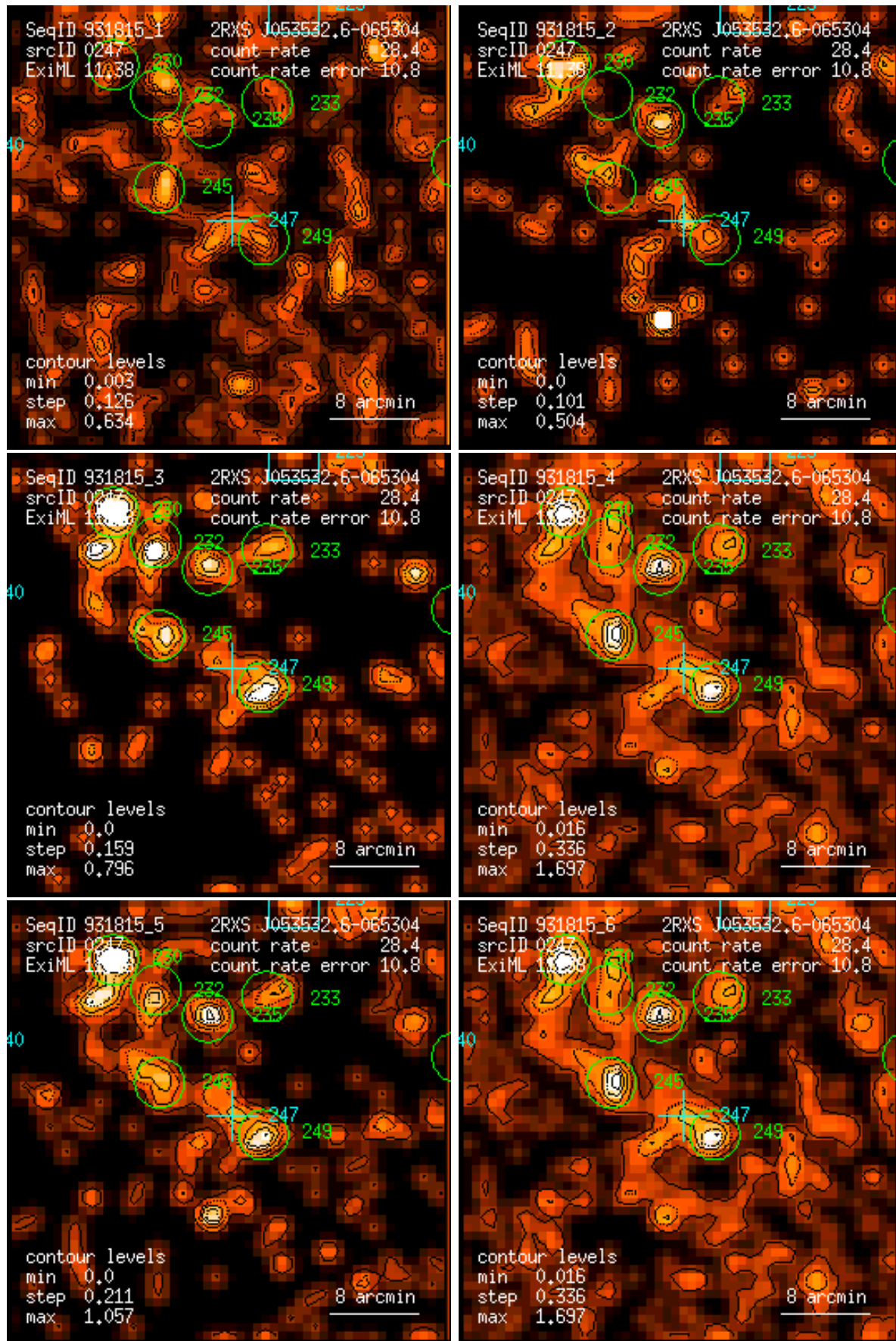
Figure 247: RASS 931815: detection 0247: band rate images, Gaussian filter: (1) PSPC channels 11 – 41, (2) 52 – 90, (3) 91 – 201, (4) 11 – 235, (5) 52 – 201, (6) 11 – 201. Broad band rates in counts/ks. Band rate contour levels in counts/ks/arcmin 2 .
