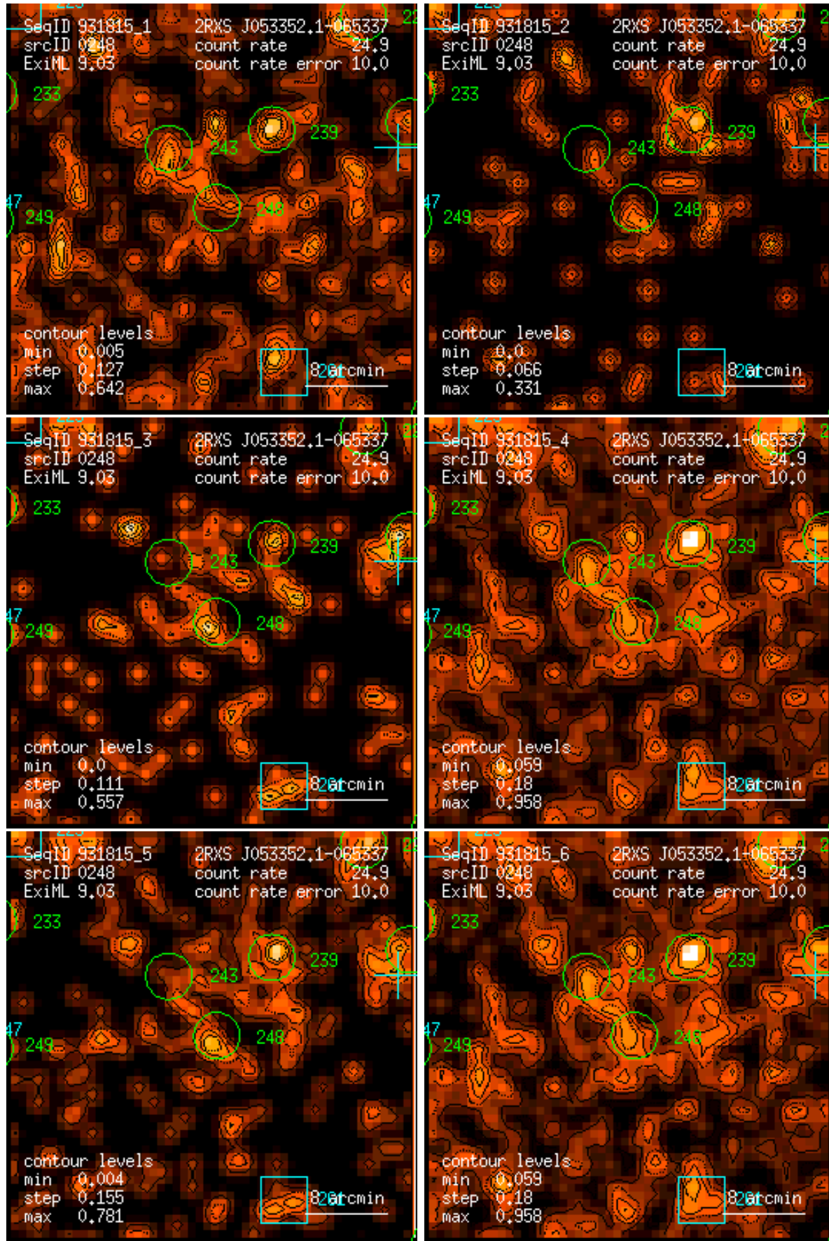
Figure 248: RASS 931815: detection 0248: band rate images, Gaussian filter: (1) PSPC channels 11 – 41, (2) 52 – 90, (3) 91 – 201, (4) 11 – 235, (5) 52 – 201, (6) 11 – 201. Broad band rates in counts/ks. Band rate contour levels in counts/ks/arcmin 2 .
