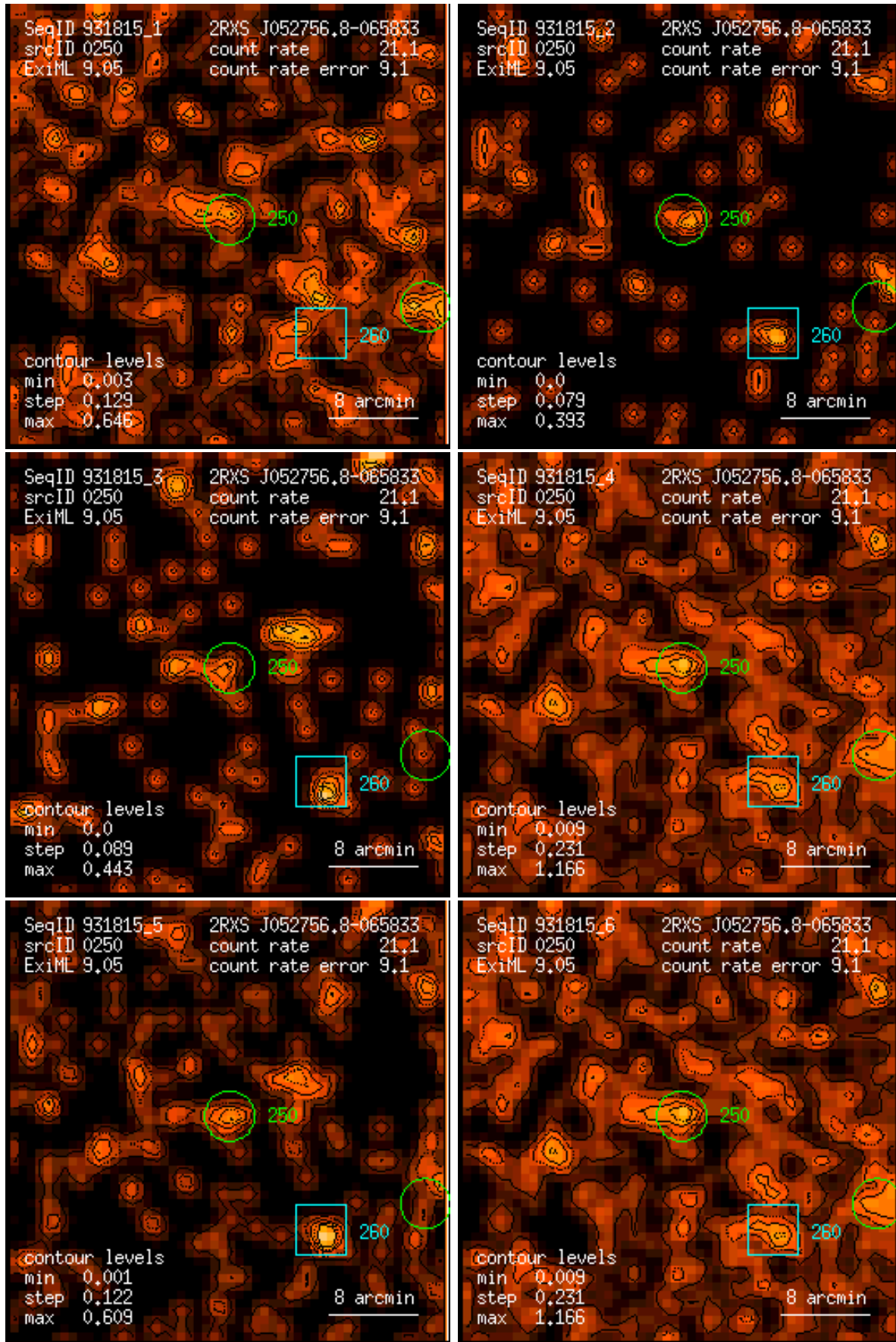
Figure 250: RASS 931815: detection 0250: band rate images, Gaussian filter: (1) PSPC channels 11 – 41, (2) 52 – 90, (3) 91 – 201, (4) 11 – 235, (5) 52 – 201, (6) 11 – 201. Broad band rates in counts/ks. Band rate contour levels in counts/ks/arcmin 2 .
