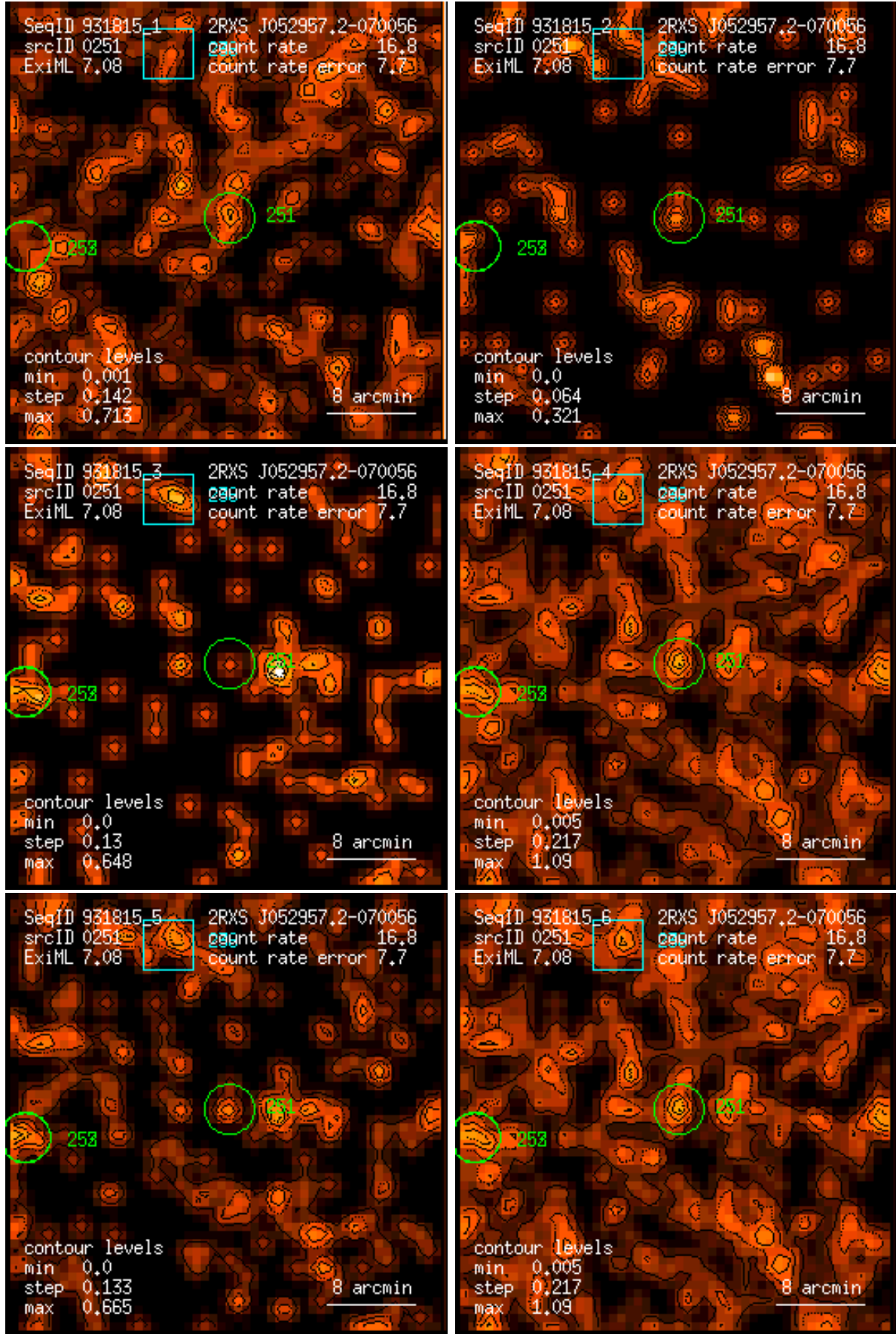
Figure 251: RASS 931815: detection 0251: band rate images, Gaussian filter: (1) PSPC channels 11 – 41, (2) 52 – 90, (3) 91 – 201, (4) 11 – 235, (5) 52 – 201, (6) 11 – 201. Broad band rates in counts/ks. Band rate contour levels in counts/ks/arcmin 2 .
