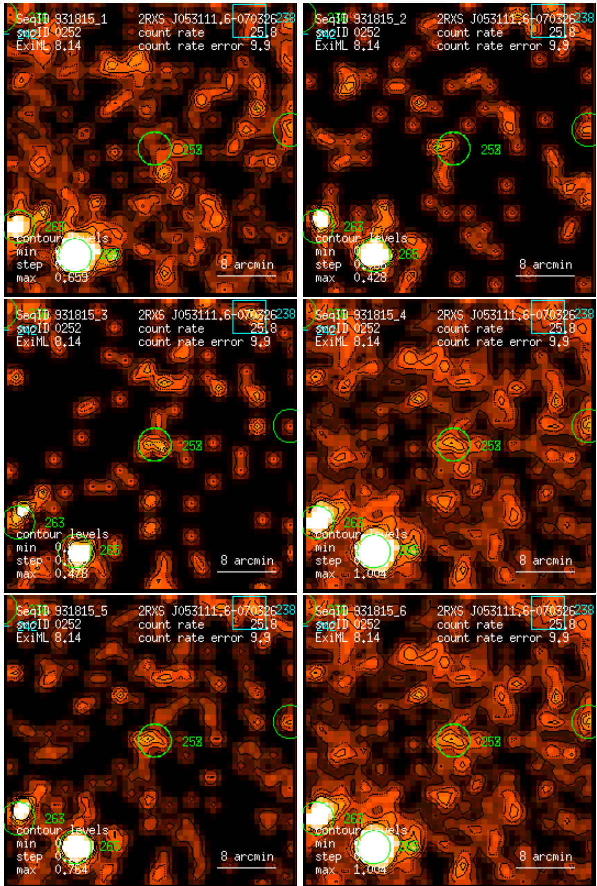
Figure 252: RASS 931815: detection 0252: band rate images, Gaussian filter: (1) PSPC channels 11 – 41, (2) 52 – 90, (3) 91 – 201, (4) 11 – 235, (5) 52 – 201, (6) 11 – 201. Broad band rates in counts/ks. Band rate contour levels in counts/ks/arcmin 2 .
