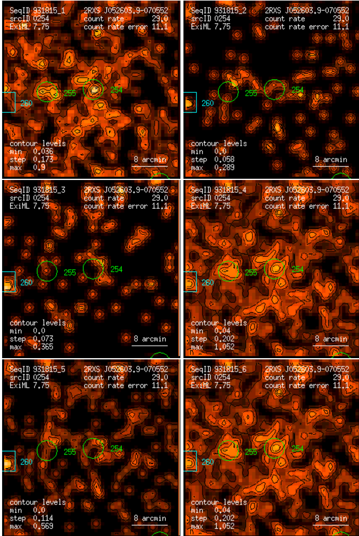
Figure 254: RASS 931815: detection 0254: band rate images, Gaussian filter: (1) PSPC channels 11 – 41, (2) 52 – 90, (3) 91 – 201, (4) 11 – 235, (5) 52 – 201, (6) 11 – 201. Broad band rates in counts/ks. Band rate contour levels in counts/ks/arcmin 2 .
