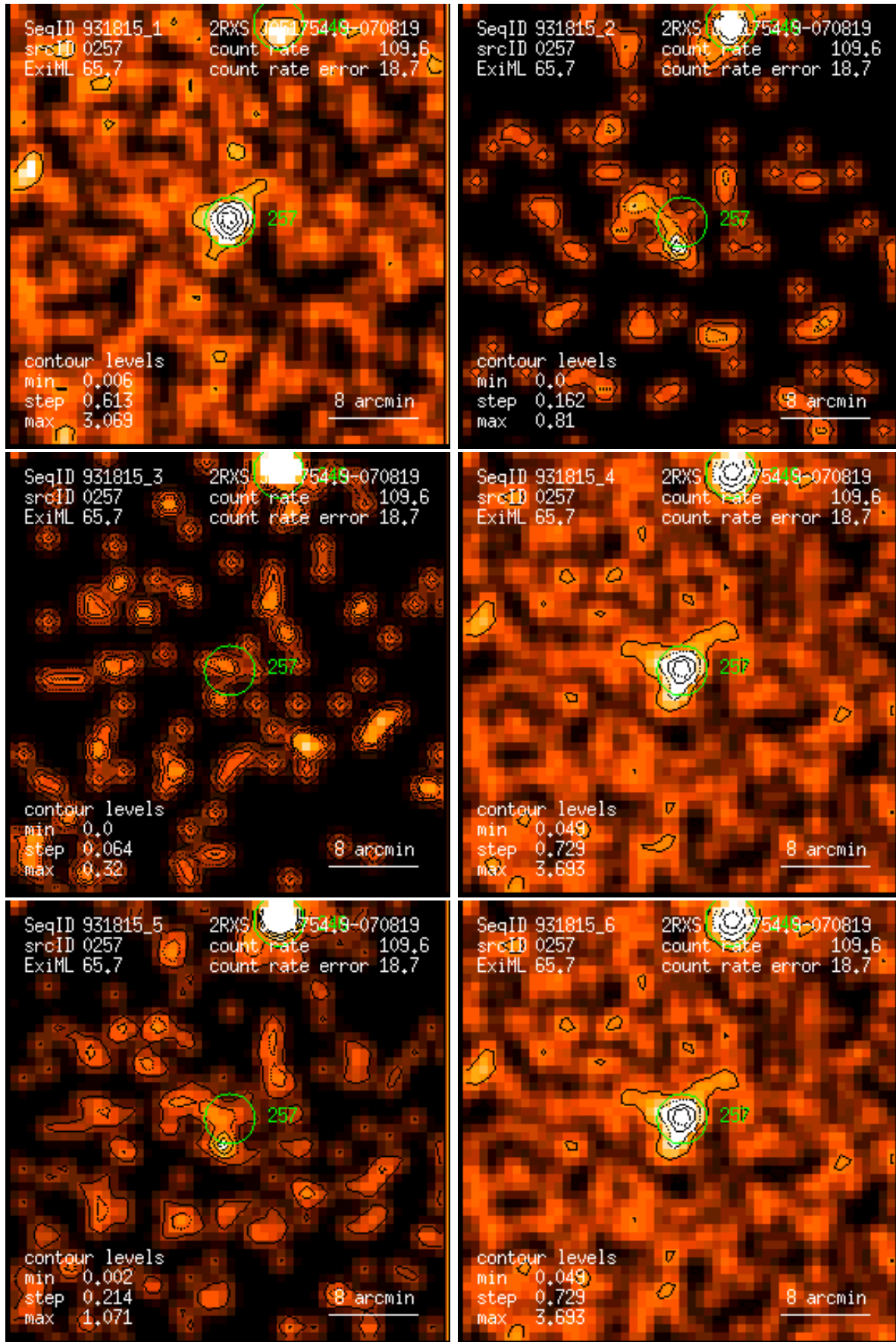
Figure 257: RASS 931815: detection 0257: band rate images, Gaussian filter: (1) PSPC channels 11 – 41, (2) 52 – 90, (3) 91 – 201, (4) 11 – 235, (5) 52 – 201, (6) 11 – 201. Broad band rates in counts/ks. Band rate contour levels in counts/ks/arcmin 2 .
