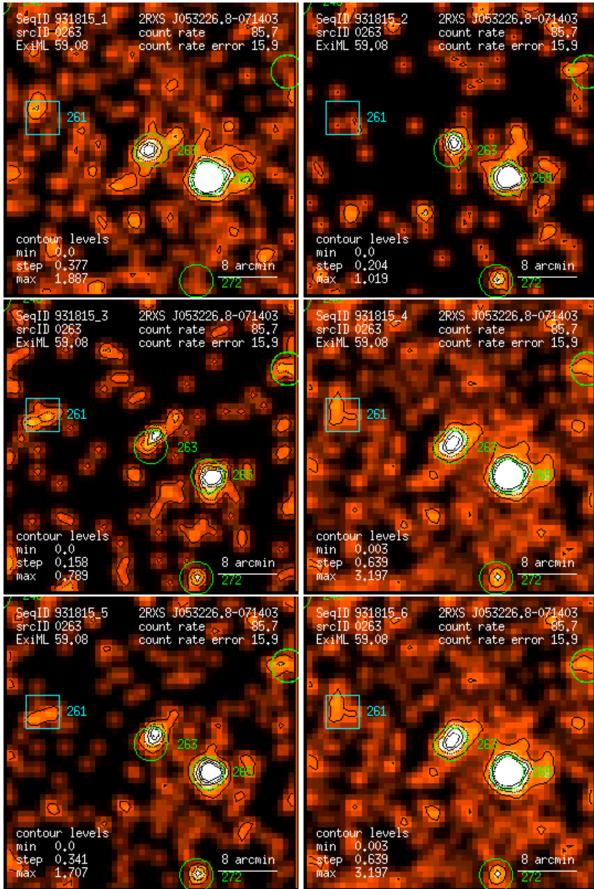
Figure 263: RASS 931815: detection 0263: band rate images, Gaussian filter: (1) PSPC channels 11 – 41, (2) 52 – 90, (3) 91 – 201, (4) 11 – 235, (5) 52 – 201, (6) 11 – 201. Broad band rates in counts/ks. Band rate contour levels in counts/ks/arcmin 2 .
