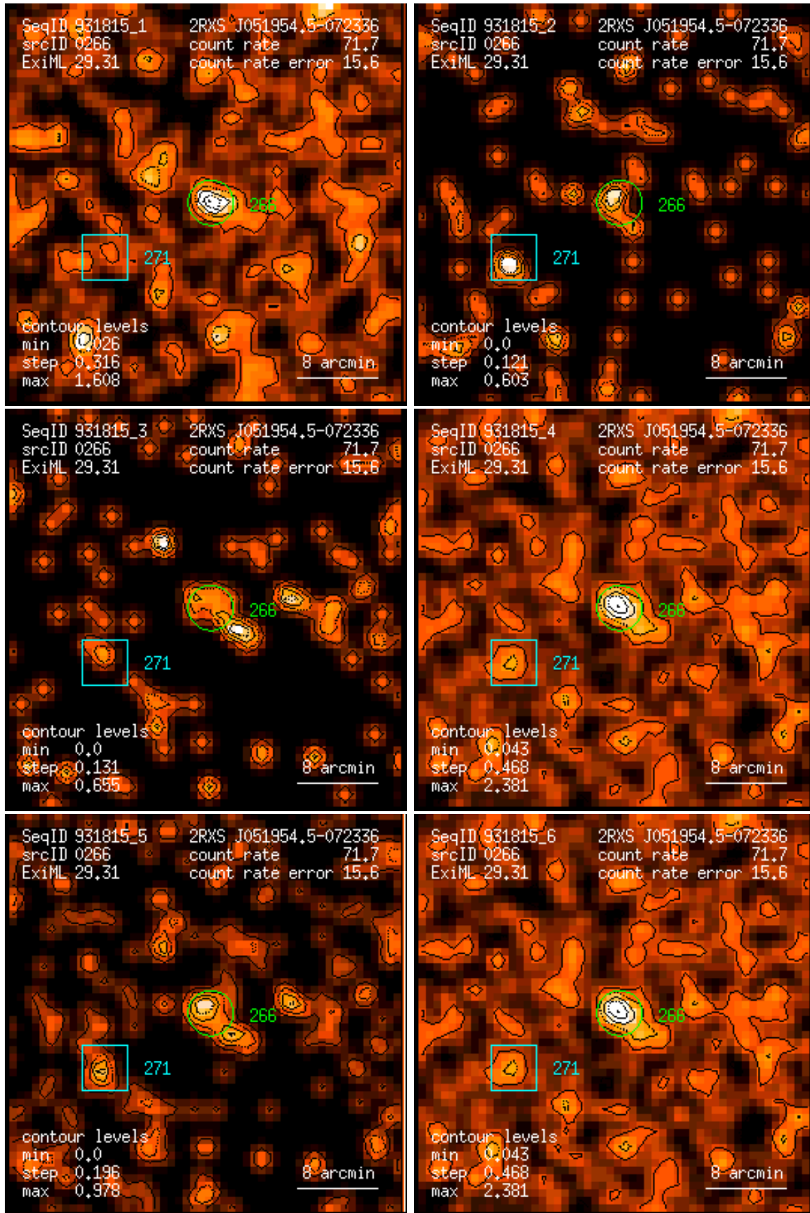
Figure 266: RASS 931815: detection 0266: band rate images, Gaussian filter: (1) PSPC channels 11 – 41, (2) 52 – 90, (3) 91 – 201, (4) 11 – 235, (5) 52 – 201, (6) 11 – 201. Broad band rates in counts/ks. Band rate contour levels in counts/ks/arcmin 2 .
