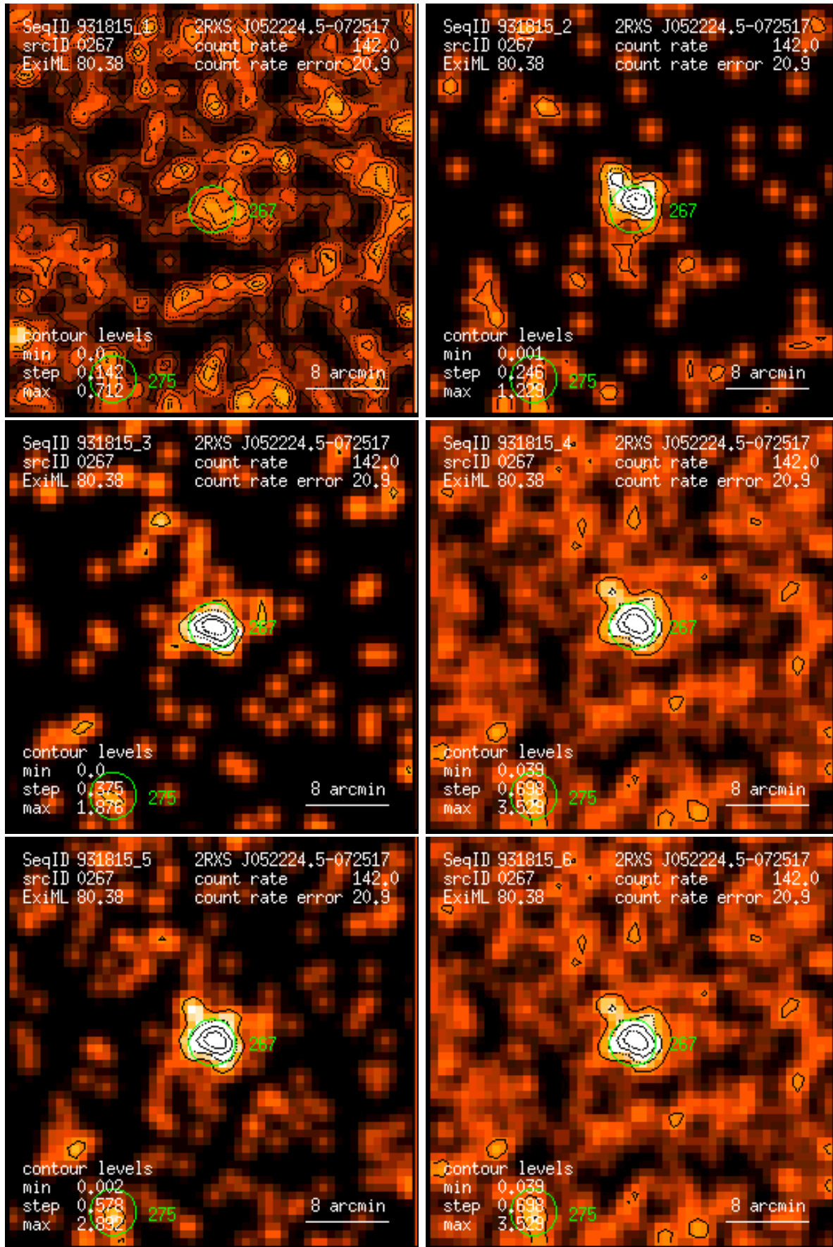
Figure 267: RASS 931815: detection 0267: band rate images, Gaussian filter: (1) PSPC channels 11 – 41, (2) 52 – 90, (3) 91 – 201, (4) 11 – 235, (5) 52 – 201, (6) 11 – 201. Broad band rates in counts/ks. Band rate contour levels in counts/ks/arcmin 2 .
