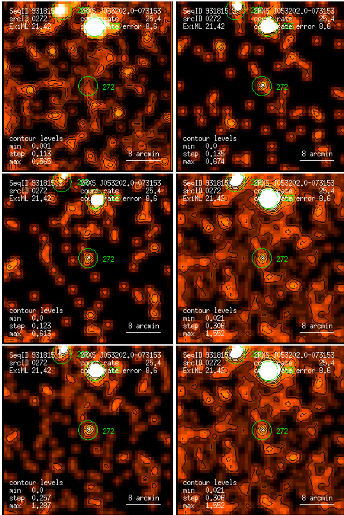
Figure 272: RASS 931815: detection 0272: band rate images, Gaussian filter: (1) PSPC channels 11 – 41, (2) 52 – 90, (3) 91 – 201, (4) 11 – 235, (5) 52 – 201, (6) 11 – 201. Broad band rates in counts/ks. Band rate contour levels in counts/ks/arcmin 2 .
