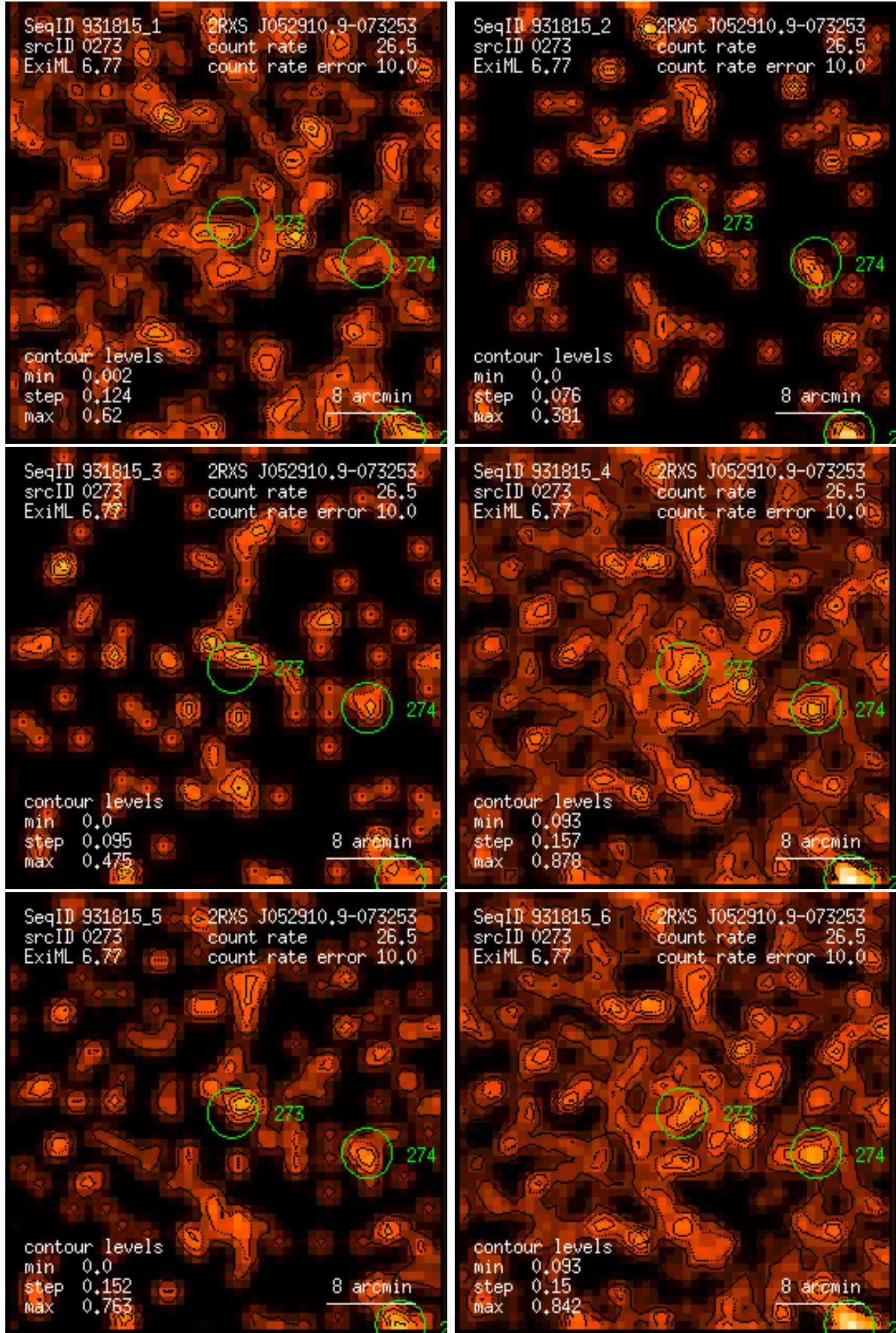
Figure 273: RASS 931815: detection 0273: band rate images, Gaussian filter: (1) PSPC channels 11 – 41, (2) 52 – 90, (3) 91 – 201, (4) 11 – 235, (5) 52 – 201, (6) 11 – 201. Broad band rates in counts/ks. Band rate contour levels in counts/ks/arcmin 2 .
