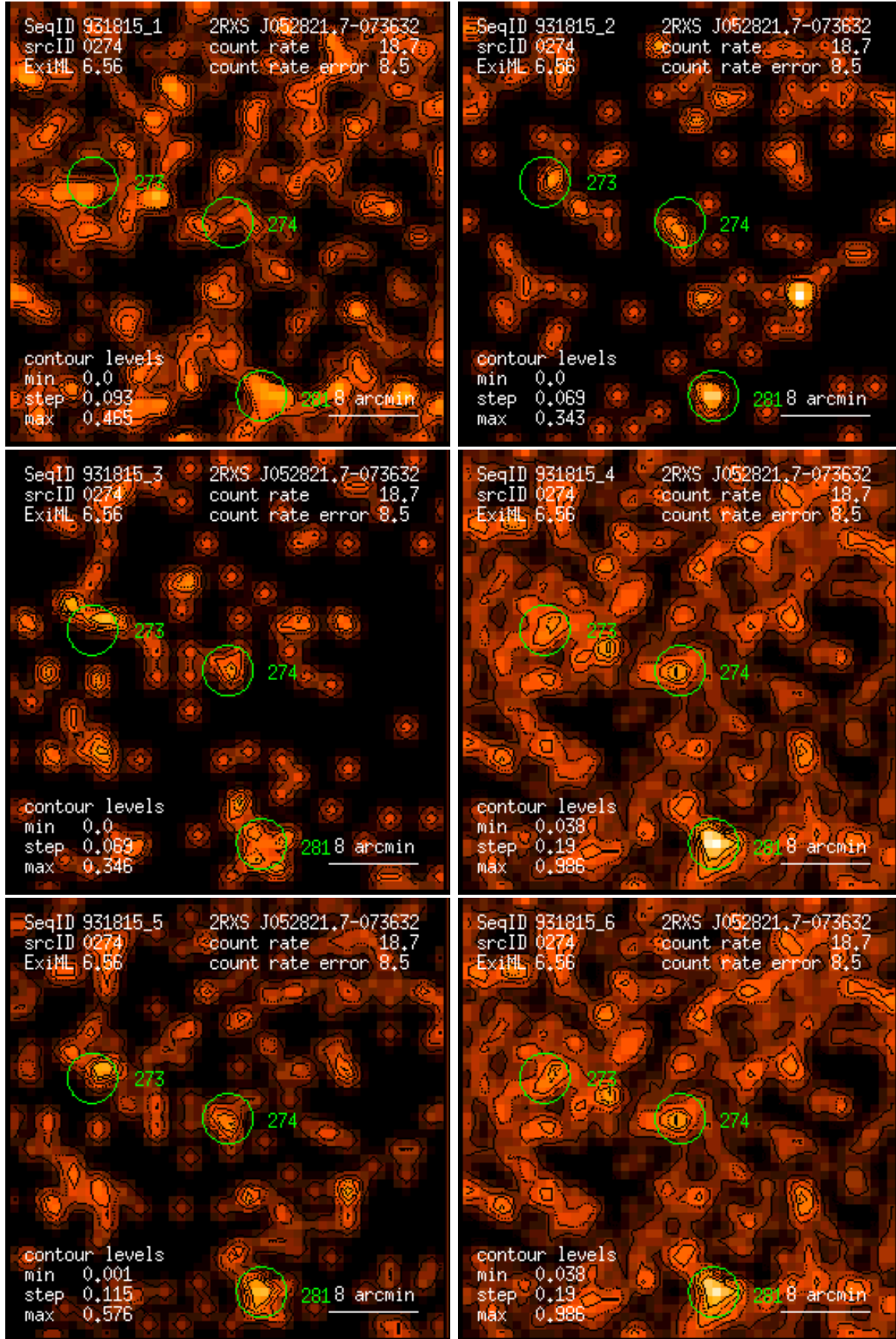
Figure 274: RASS 931815: detection 0274: band rate images, Gaussian filter: (1) PSPC channels 11 – 41, (2) 52 – 90, (3) 91 – 201, (4) 11 – 235, (5) 52 – 201, (6) 11 – 201. Broad band rates in counts/ks. Band rate contour levels in counts/ks/arcmin 2 .
