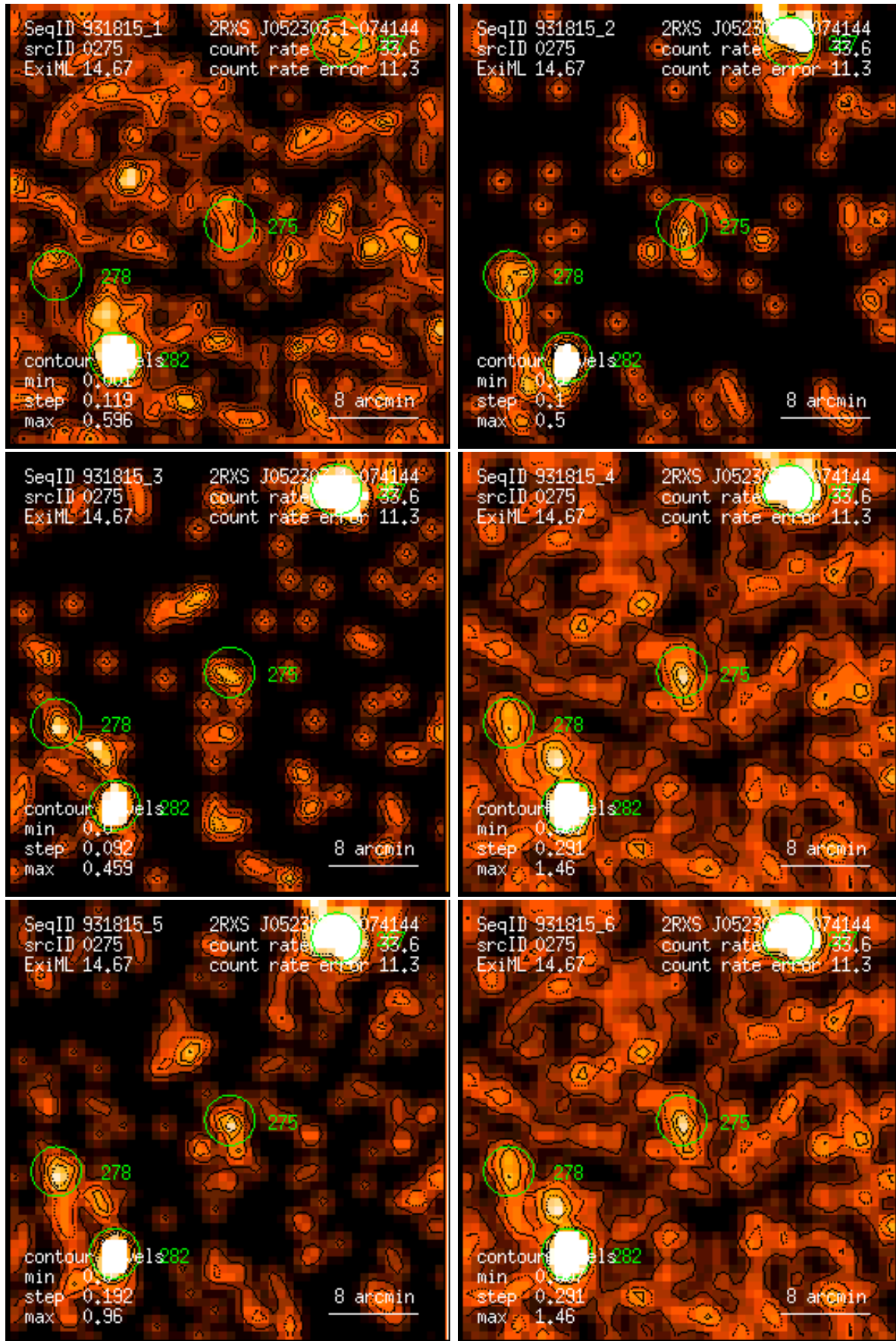
Figure 275: RASS 931815: detection 0275: band rate images, Gaussian filter: (1) PSPC channels 11 – 41, (2) 52 – 90, (3) 91 – 201, (4) 11 – 235, (5) 52 – 201, (6) 11 – 201. Broad band rates in counts/ks. Band rate contour levels in counts/ks/arcmin 2 .
