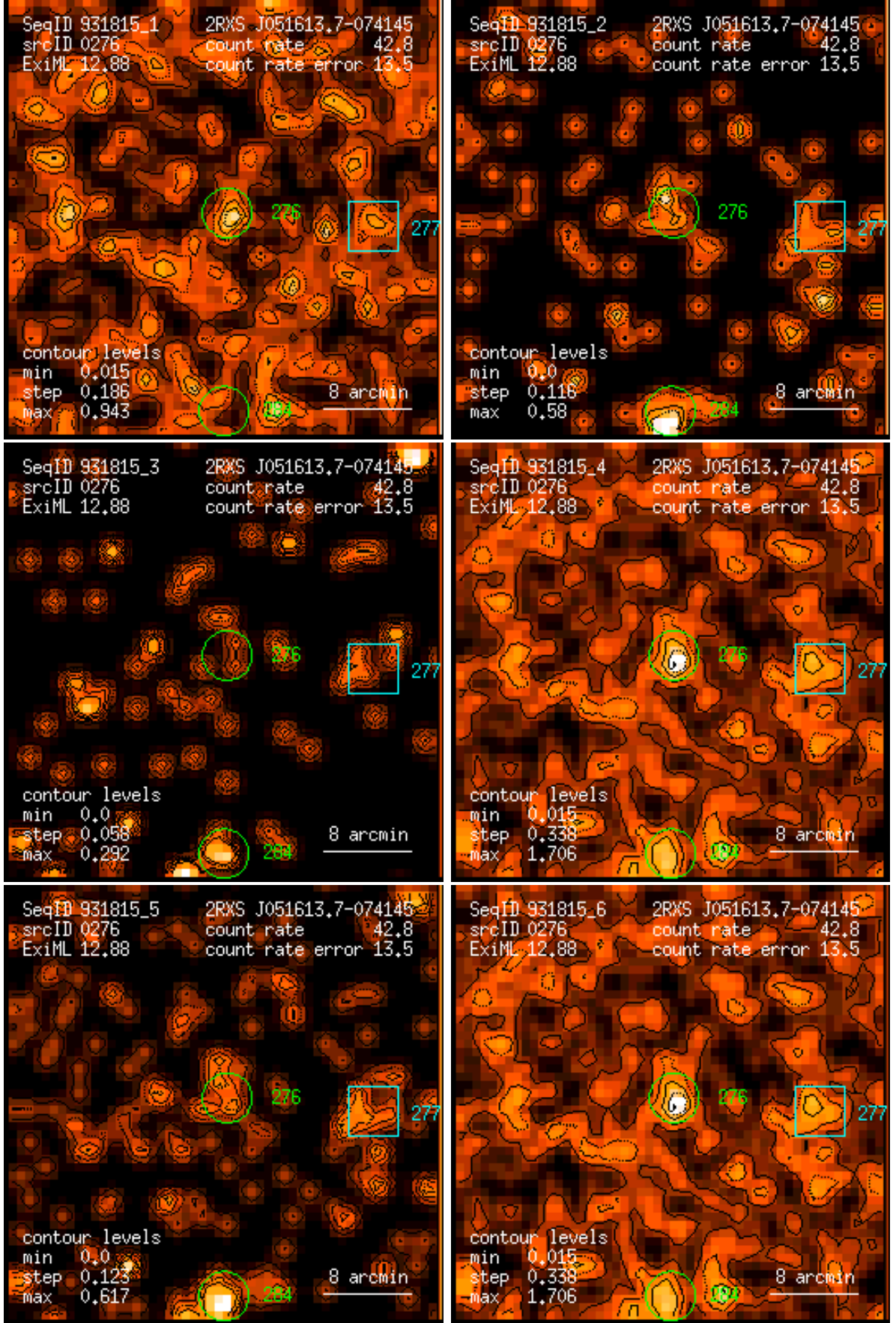
Figure 276: RASS 931815: detection 0276: band rate images, Gaussian filter: (1) PSPC channels 11 – 41, (2) 52 – 90, (3) 91 – 201, (4) 11 – 235, (5) 52 – 201, (6) 11 – 201. Broad band rates in counts/ks. Band rate contour levels in counts/ks/arcmin 2 .
