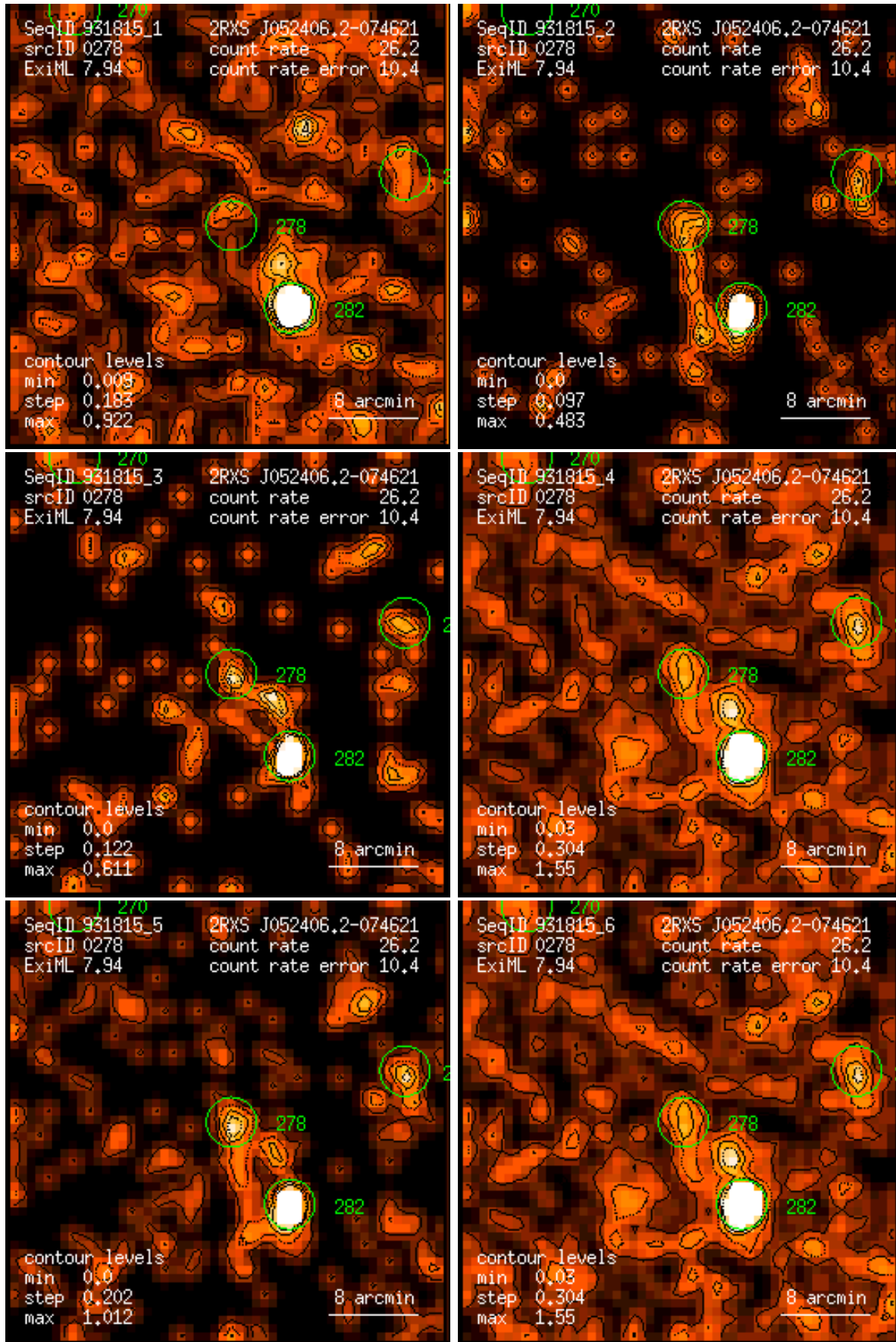
Figure 278: RASS 931815: detection 0278: band rate images, Gaussian filter: (1) PSPC channels 11 – 41, (2) 52 – 90, (3) 91 – 201, (4) 11 – 235, (5) 52 – 201, (6) 11 – 201. Broad band rates in counts/ks. Band rate contour levels in counts/ks/arcmin 2 .
