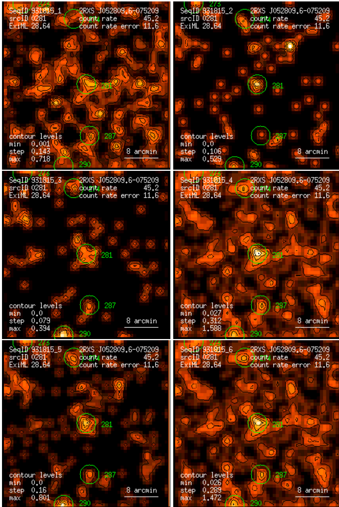
Figure 281: RASS 931815: detection 0281: band rate images, Gaussian filter: (1) PSPC channels 11 – 41, (2) 52 – 90, (3) 91 – 201, (4) 11 – 235, (5) 52 – 201, (6) 11 – 201. Broad band rates in counts/ks. Band rate contour levels in counts/ks/arcmin 2 .
