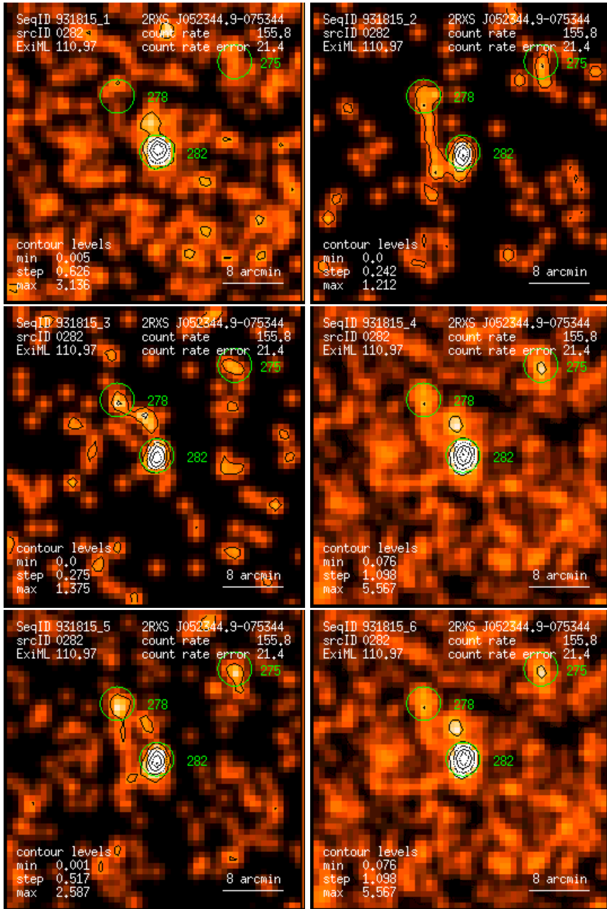
Figure 282: RASS 931815: detection 0282: band rate images, Gaussian filter: (1) PSPC channels 11 – 41, (2) 52 – 90, (3) 91 – 201, (4) 11 – 235, (5) 52 – 201, (6) 11 – 201. Broad band rates in counts/ks. Band rate contour levels in counts/ks/arcmin 2 .
