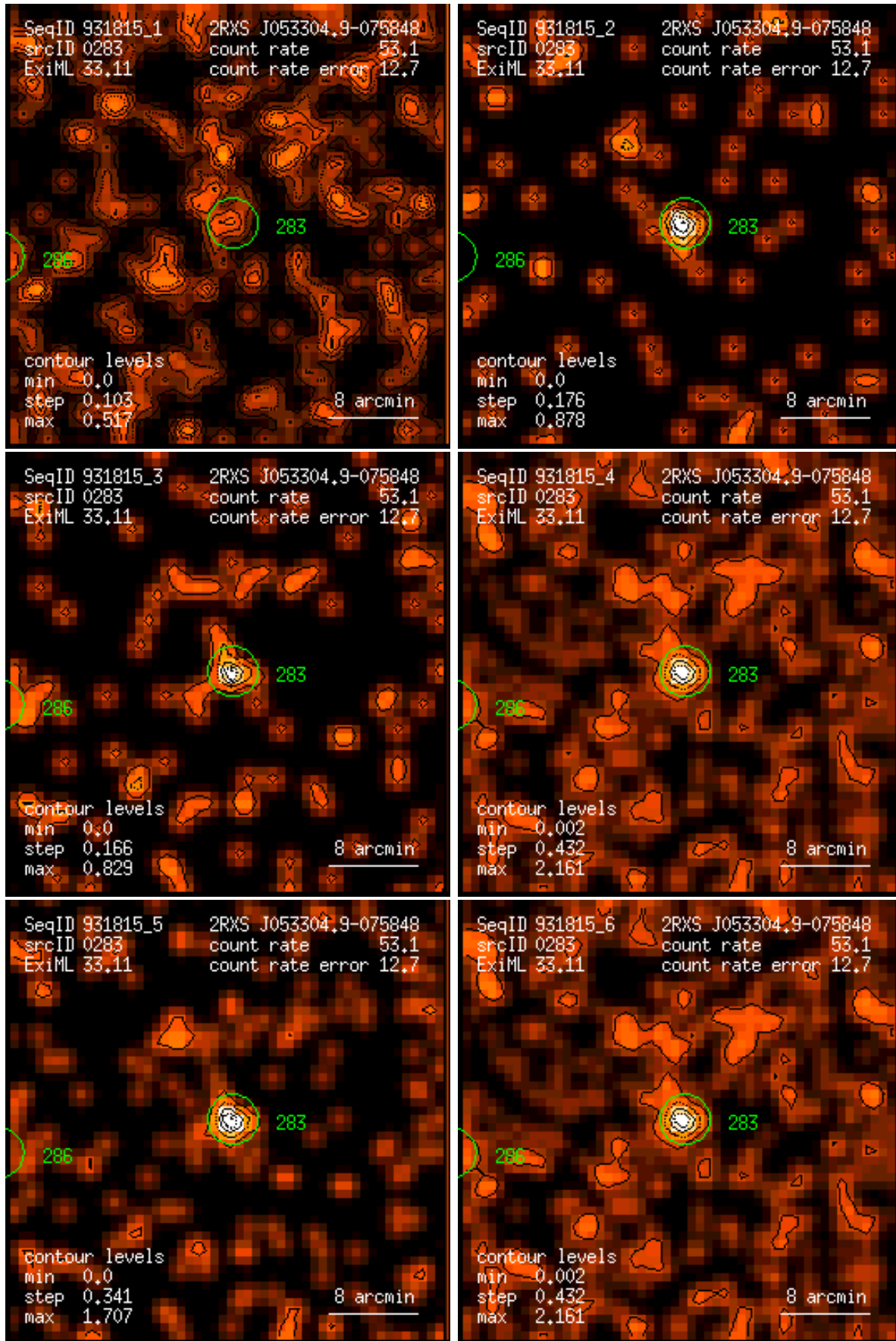
Figure 283: RASS 931815: detection 0283: band rate images, Gaussian filter: (1) PSPC channels 11 – 41, (2) 52 – 90, (3) 91 – 201, (4) 11 – 235, (5) 52 – 201, (6) 11 – 201. Broad band rates in counts/ks. Band rate contour levels in counts/ks/arcmin 2 .
