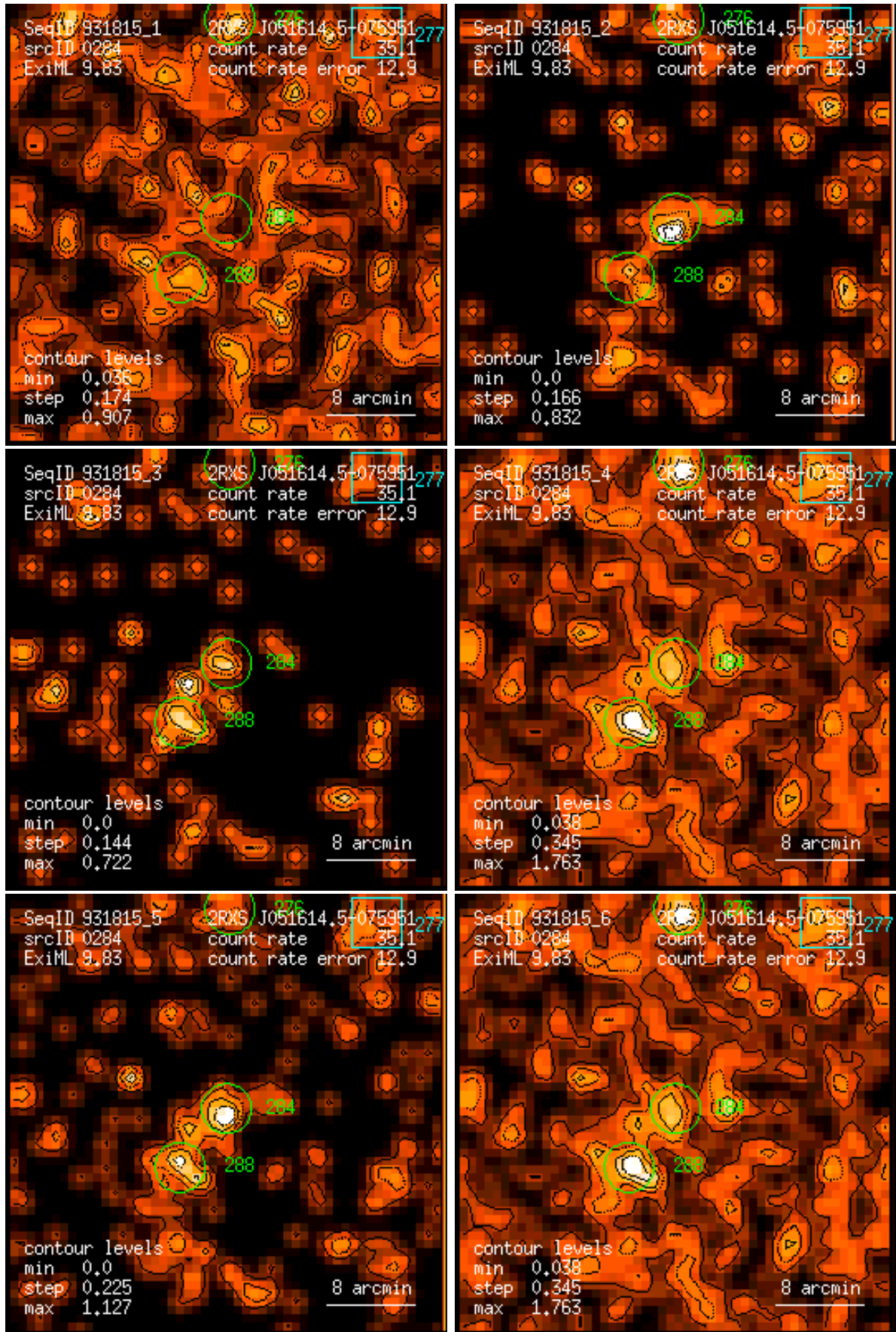
Figure 284: RASS 931815: detection 0284: band rate images, Gaussian filter: (1) PSPC channels 11 – 41, (2) 52 – 90, (3) 91 – 201, (4) 11 – 235, (5) 52 – 201, (6) 11 – 201. Broad band rates in counts/ks. Band rate contour levels in counts/ks/arcmin 2 .
