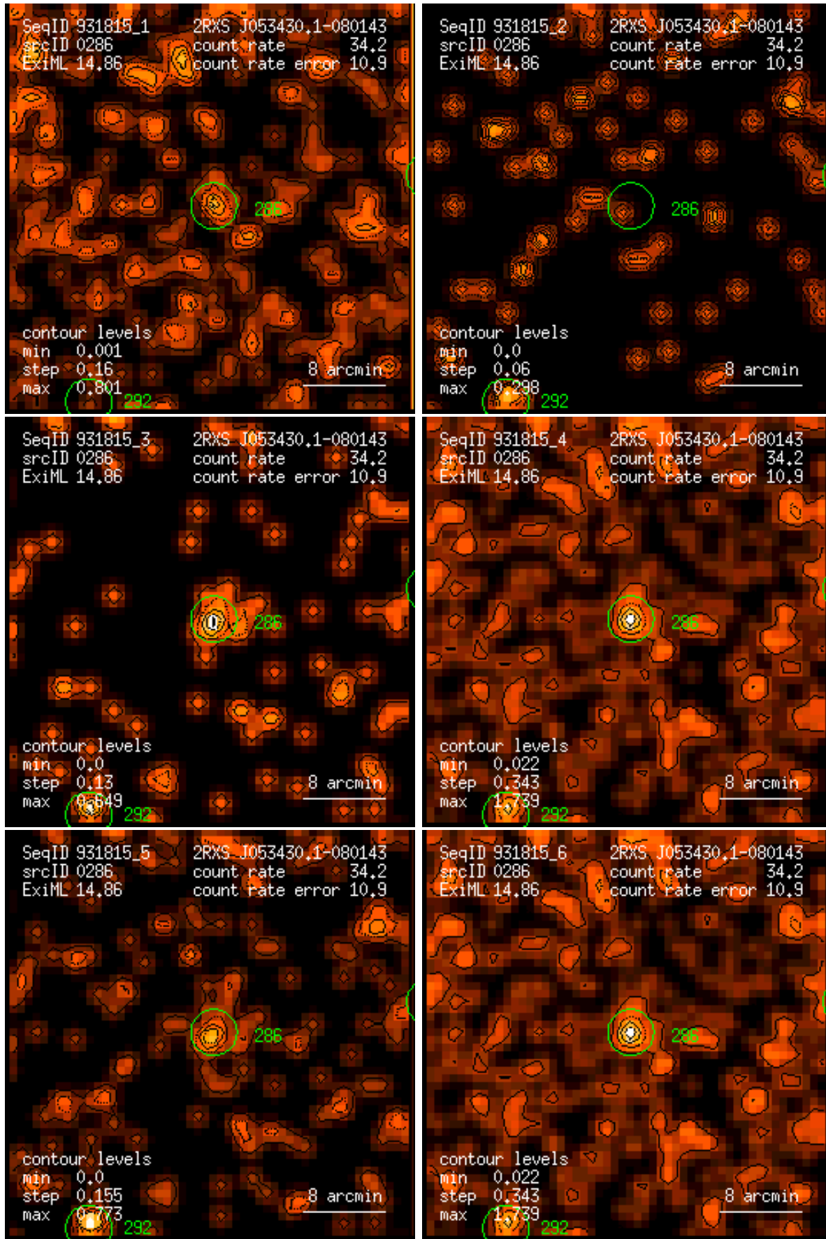
Figure 286: RASS 931815: detection 0286: band rate images, Gaussian filter: (1) PSPC channels 11 – 41, (2) 52 – 90, (3) 91 – 201, (4) 11 – 235, (5) 52 – 201, (6) 11 – 201. Broad band rates in counts/ks. Band rate contour levels in counts/ks/arcmin 2 .
