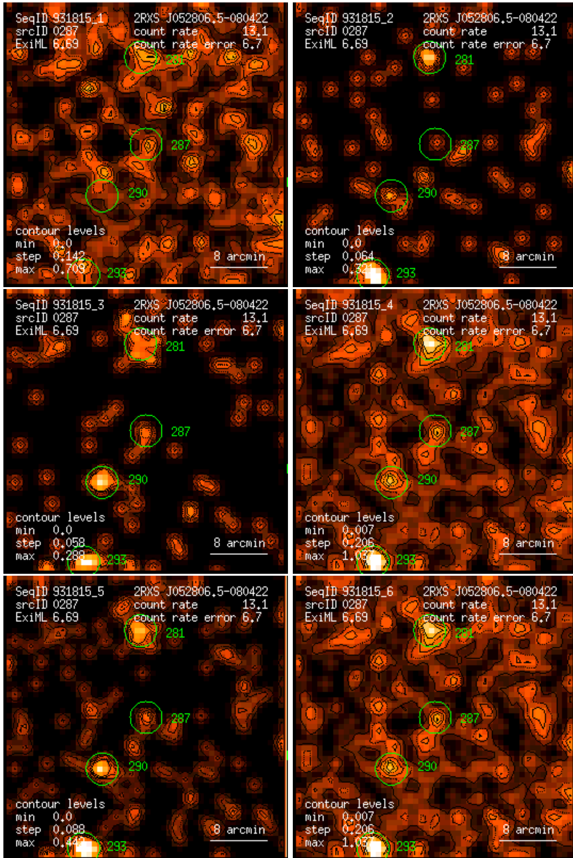
Figure 287: RASS 931815: detection 0287: band rate images, Gaussian filter: (1) PSPC channels 11 – 41, (2) 52 – 90, (3) 91 – 201, (4) 11 – 235, (5) 52 – 201, (6) 11 – 201. Broad band rates in counts/ks. Band rate contour levels in counts/ks/arcmin 2 .
