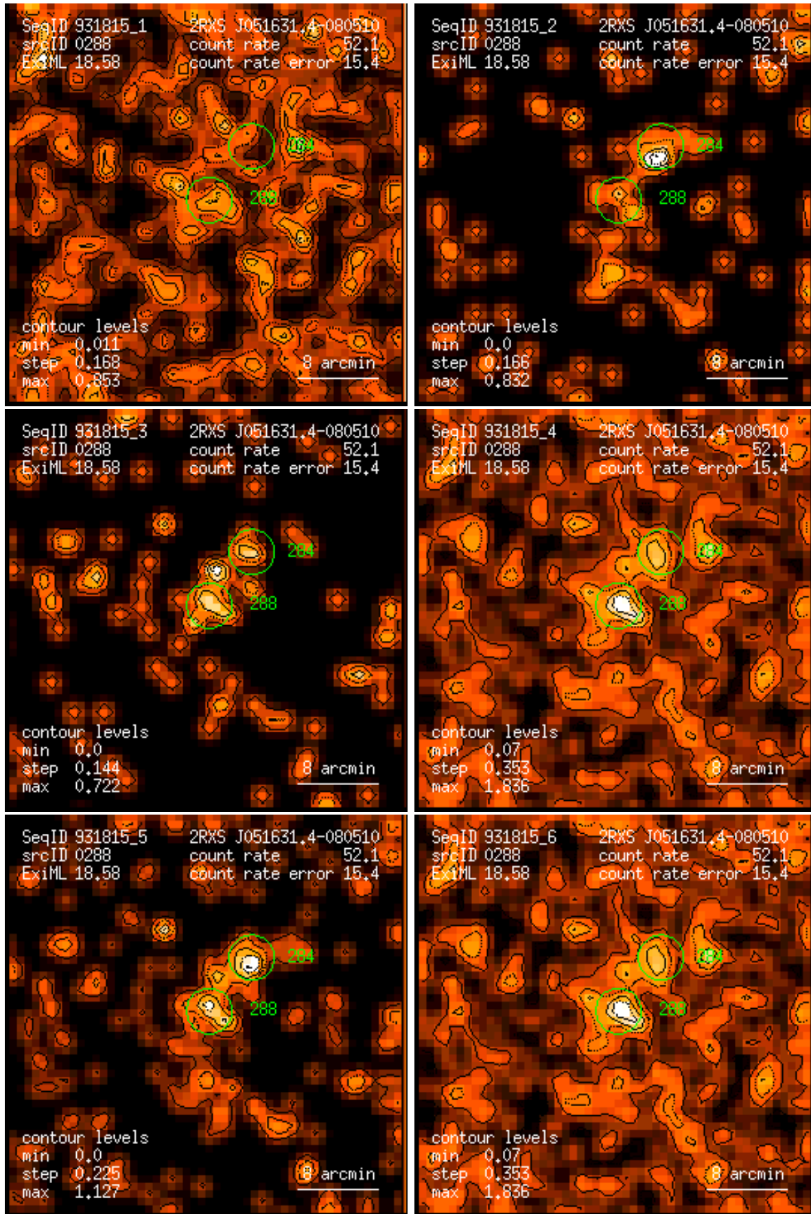
Figure 288: RASS 931815: detection 0288: band rate images, Gaussian filter: (1) PSPC channels 11 – 41, (2) 52 – 90, (3) 91 – 201, (4) 11 – 235, (5) 52 – 201, (6) 11 – 201. Broad band rates in counts/ks. Band rate contour levels in counts/ks/arcmin 2 .
