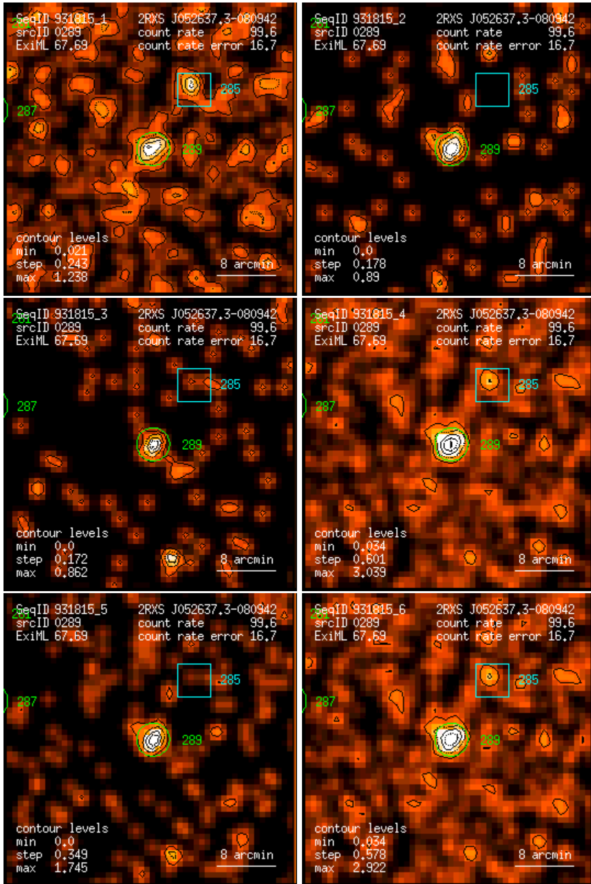
Figure 289: RASS 931815: detection 0289: band rate images, Gaussian filter: (1) PSPC channels 11 – 41, (2) 52 – 90, (3) 91 – 201, (4) 11 – 235, (5) 52 – 201, (6) 11 – 201. Broad band rates in counts/ks. Band rate contour levels in counts/ks/arcmin 2 .
