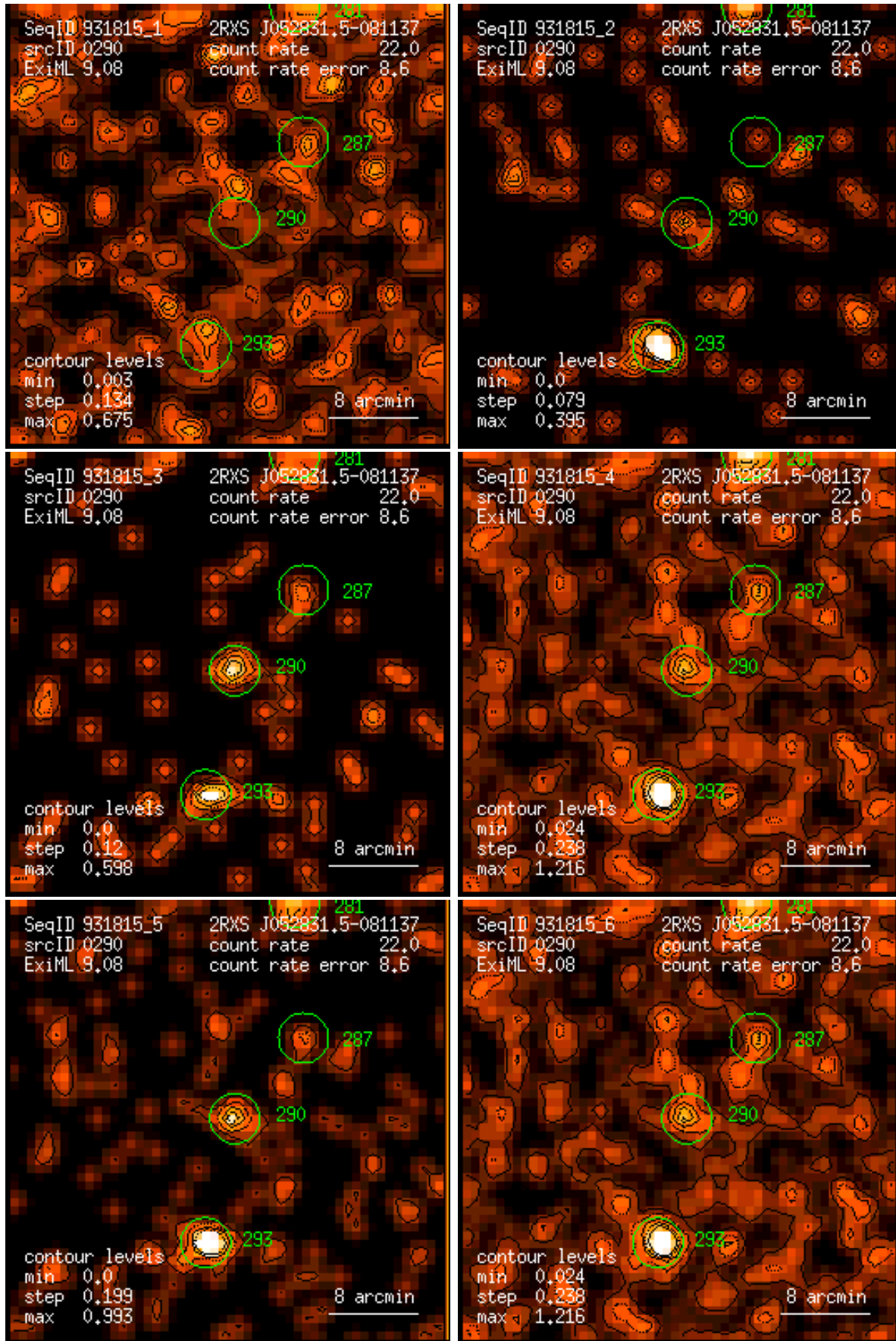
Figure 290: RASS 931815: detection 0290: band rate images, Gaussian filter: (1) PSPC channels 11 – 41, (2) 52 – 90, (3) 91 – 201, (4) 11 – 235, (5) 52 – 201, (6) 11 – 201. Broad band rates in counts/ks. Band rate contour levels in counts/ks/arcmin 2 .
