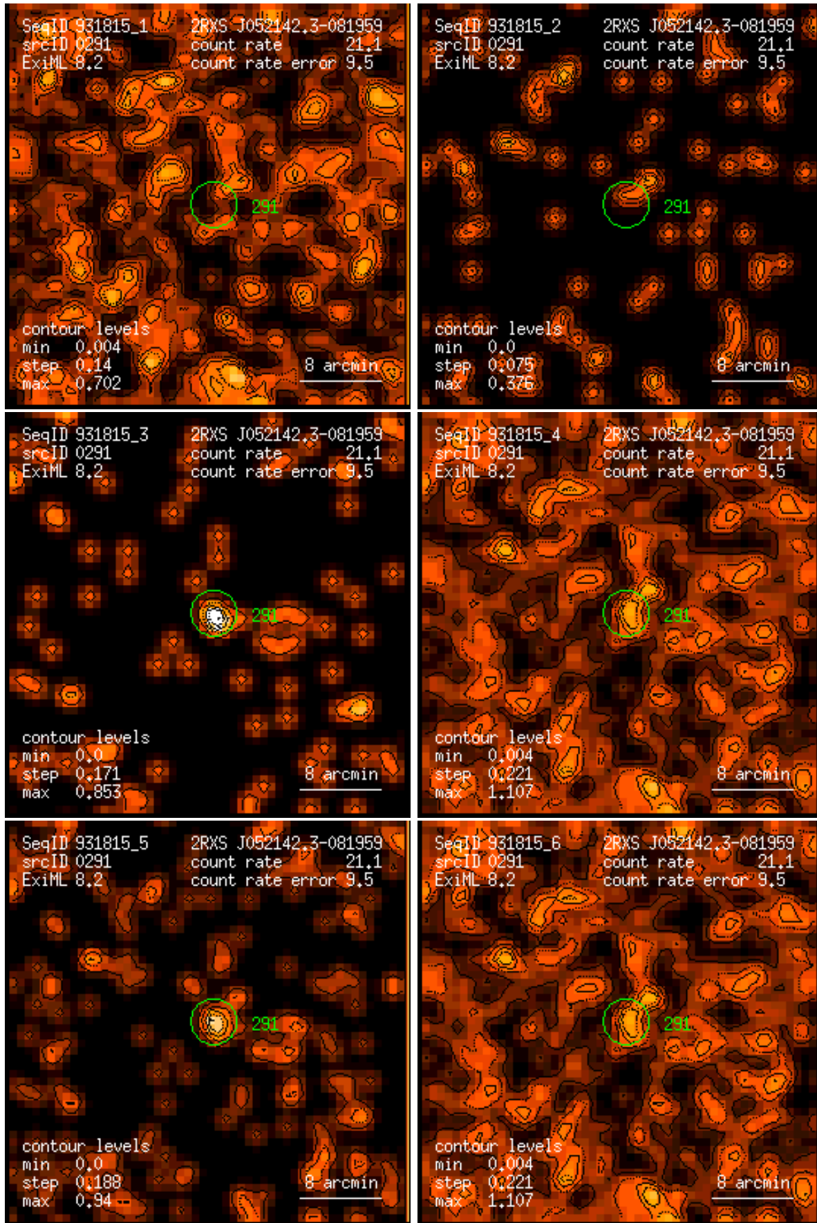
Figure 291: RASS 931815: detection 0291: band rate images, Gaussian filter: (1) PSPC channels 11 – 41, (2) 52 – 90, (3) 91 – 201, (4) 11 – 235, (5) 52 – 201, (6) 11 – 201. Broad band rates in counts/ks. Band rate contour levels in counts/ks/arcmin 2 .
