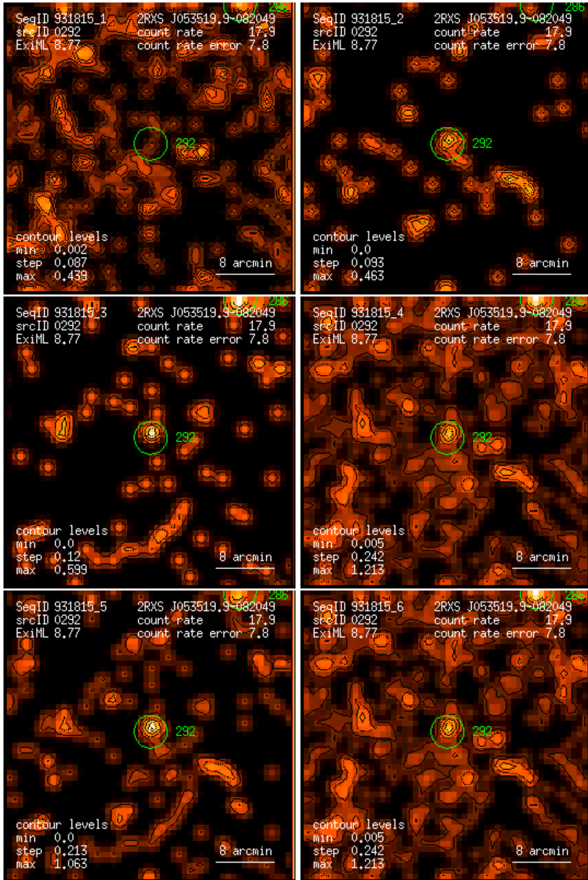
Figure 292: RASS 931815: detection 0292: band rate images, Gaussian filter: (1) PSPC channels 11 – 41, (2) 52 – 90, (3) 91 – 201, (4) 11 – 235, (5) 52 – 201, (6) 11 – 201. Broad band rates in counts/ks. Band rate contour levels in counts/ks/arcmin 2 .
