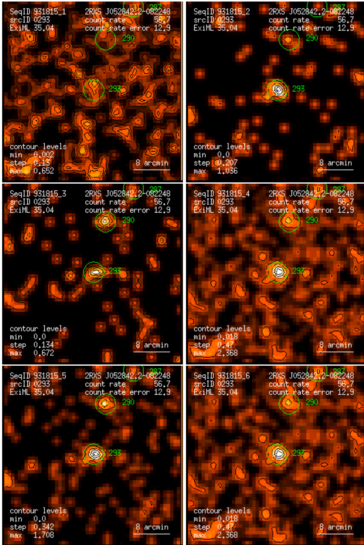
Figure 293: RASS 931815: detection 0293: band rate images, Gaussian filter: (1) PSPC channels 11 – 41, (2) 52 – 90, (3) 91 – 201, (4) 11 – 235, (5) 52 – 201, (6) 11 – 201. Broad band rates in counts/ks. Band rate contour levels in counts/ks/arcmin 2 .
