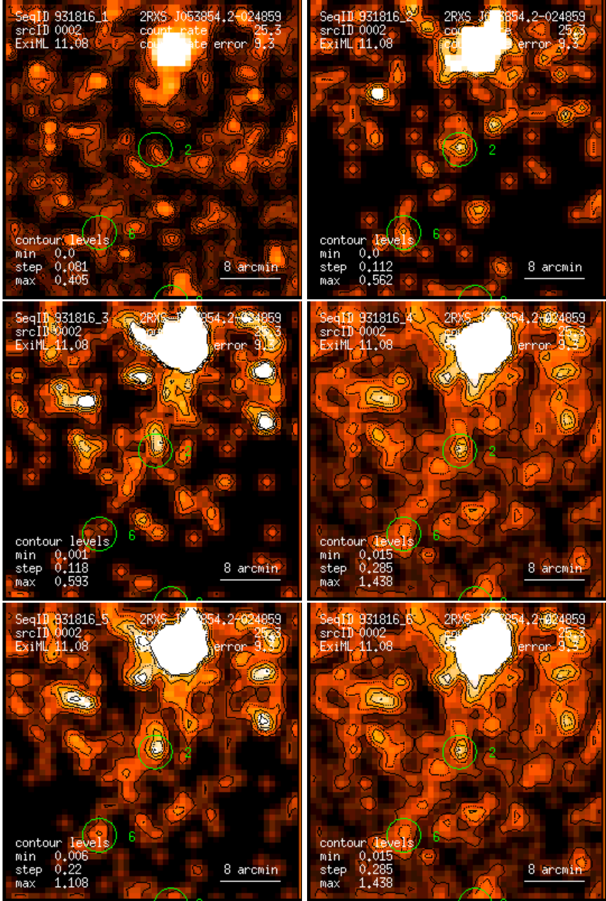
Figure 2: RASS 931816: detection 0002: band rate images, Gaussian filter: (1) PSPC channels 11 – 41, (2) 52 – 90, (3) 91 – 201, (4) 11 – 235, (5) 52 – 201, (6) 11 – 201. Broad band rates in counts/ks. Band rate contour levels in counts/ks/arcmin 2 .
