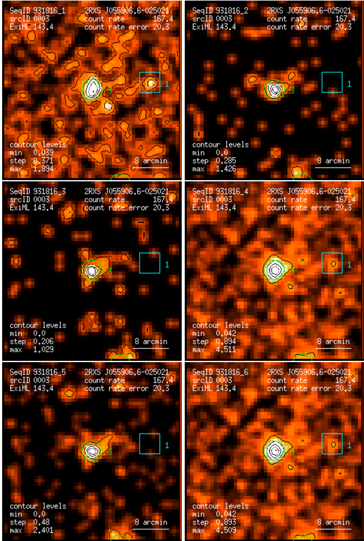
Figure 3: RASS 931816: detection 0003: band rate images, Gaussian filter: (1) PSPC channels 11 – 41, (2) 52 – 90, (3) 91 – 201, (4) 11 – 235, (5) 52 – 201, (6) 11 – 201. Broad band rates in counts/ks. Band rate contour levels in counts/ks/arcmin 2 .
