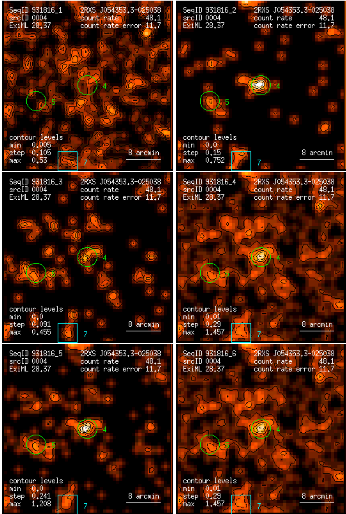
Figure 4: RASS 931816: detection 0004: band rate images, Gaussian filter: (1) PSPC channels 11 – 41, (2) 52 – 90, (3) 91 – 201, (4) 11 – 235, (5) 52 – 201, (6) 11 – 201. Broad band rates in counts/ks. Band rate contour levels in counts/ks/arcmin 2 .
